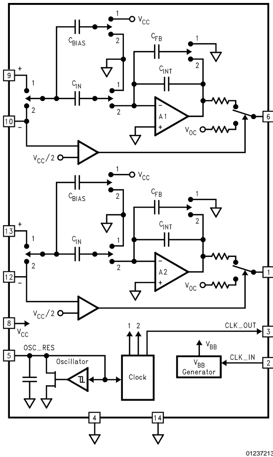
FIGURE 3. Simplified Circuit
