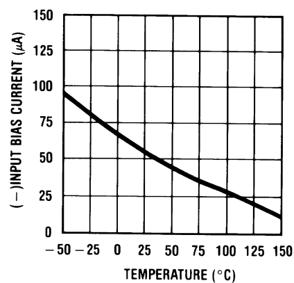
Inverting Input Bias Current vs Temperature
