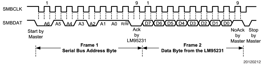
(c) Serial Bus byte Read from a Register with the internal Command Register preset to desired value.
