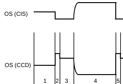
Figure 2: CIS vs. CCD Output signals
