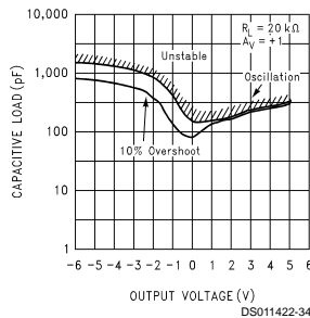
Stability vs Capacitive Load, R_L = 20 k\Omega
