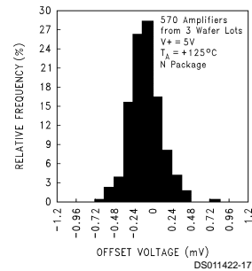
Distribution of LMC6061 Input Offset Voltage ( T_A = +125^\circ\text{C} )
