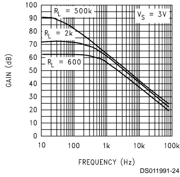
Open Loop Frequency Response (3V)
