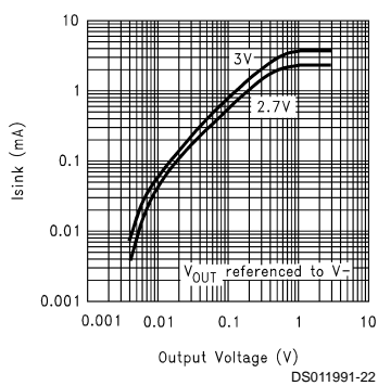
Sinking Current vs Output Voltage (2.7V)
