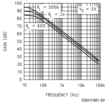
Open Loop Frequency Response (5V)
