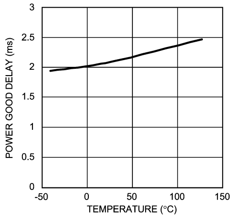
Power Good Delay vs. Temperature ( V_{IN} = 3.3V )
