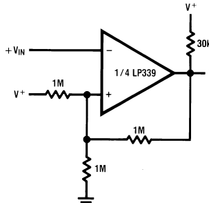
Inverting Comparator with Hysteresis
