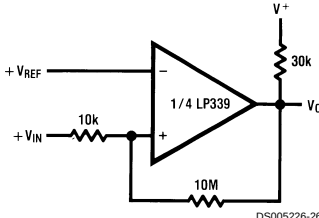
Non-Inverting Comparator with Hysteresis
