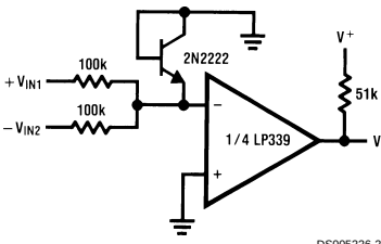
Comparing Input Voltages of Opposite Polarity
