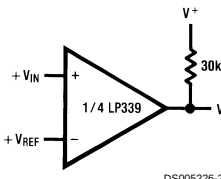
Basic Comparator
