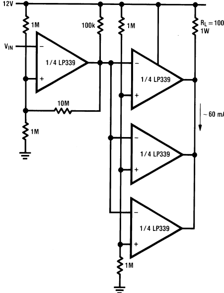
Comparator With 60 mA Sink Capability
