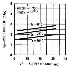
Input Current
