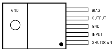
TO-220, Top View
