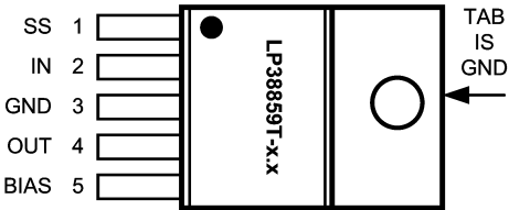
TO220-5, Top View
