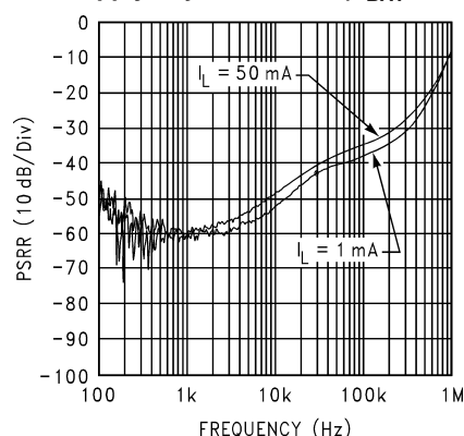
Power Supply Rejection Ratio ( V_{BAT}=3.46V )
