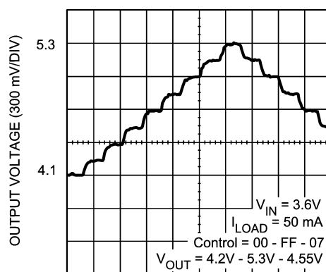
Boost Output Voltage Control
