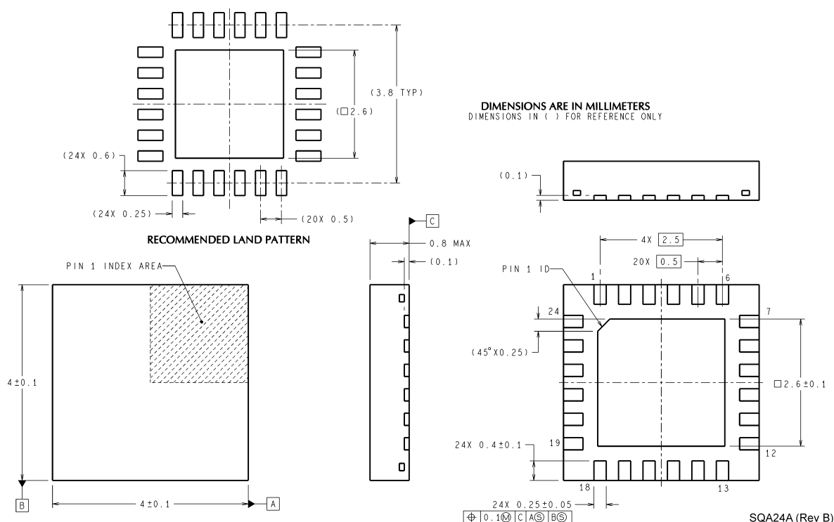
24-Lead LLP Package, 4 x 4 x 0.8 mm NS Package Number NSQAL024
