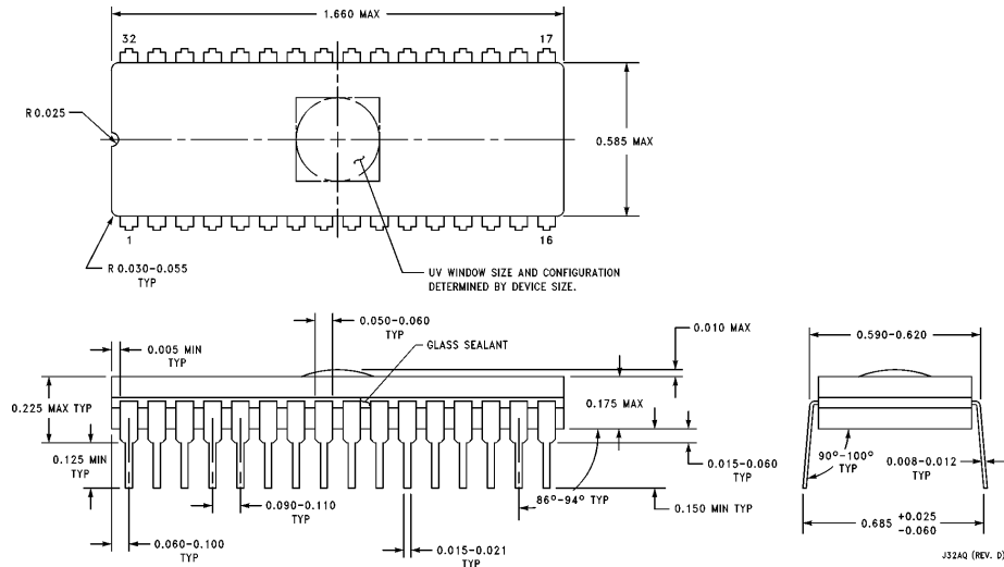
32-Lead EPROM Ceramic Dual-In-Line Package (JQ) Order Number NM27P040QXXX NS Package Number J32AQ
