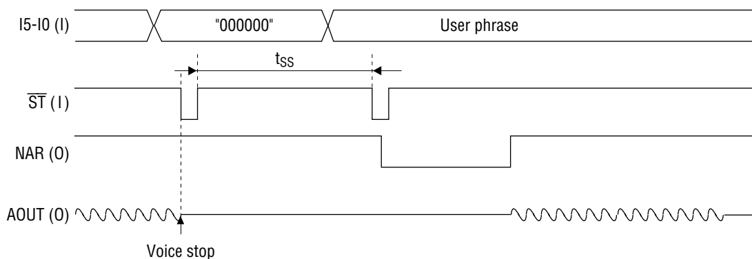
Figure 3.1 Stop Code Input Timing
