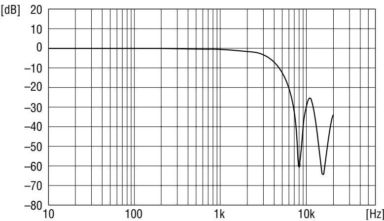
Figure. 7.1 LPF Frequency Characteristics ( f_{\text{SAM}}=8\text{ kHz} )
