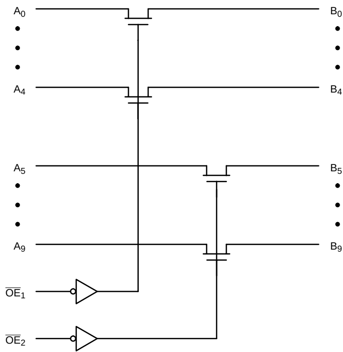
Figure 2. Logic Diagram
