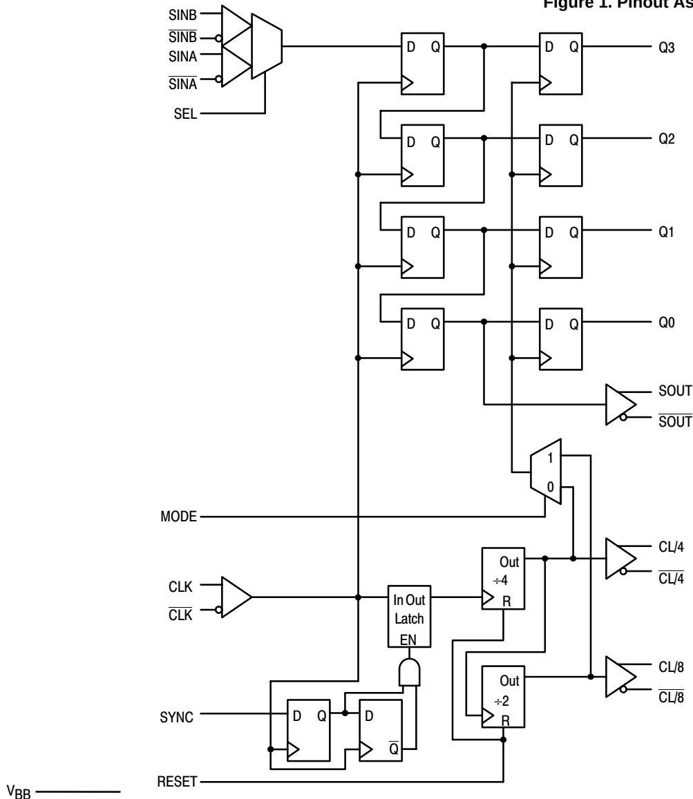
Figure 2. Logic Diagram
