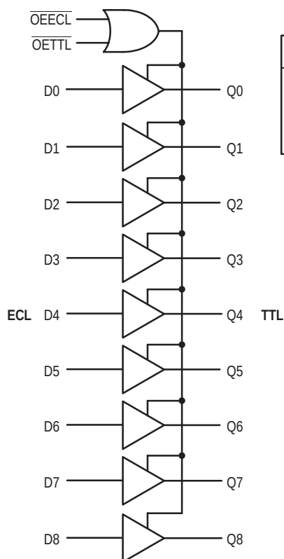
Figure 1. Logic Diagram
