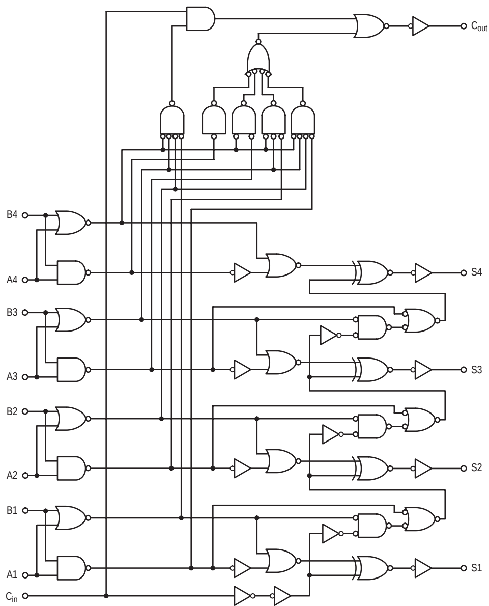
Figure 5. Logic Diagram
