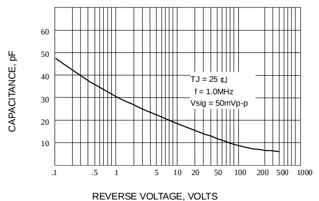
Fig. 6-TYPICAL JUNCTION CAPACITANCE
