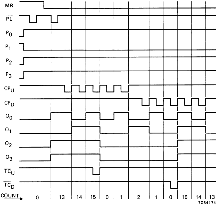
Fig.7 Timing diagram.
