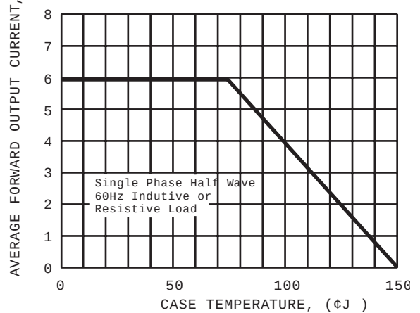
FIG. 2 - TYPICAL FORWARD CURRENT DERATING
