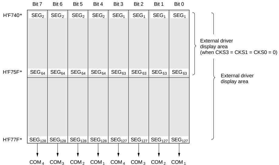
Figure 13-11 LCD RAM Map When All External Segments are Used (Example: SGX = 1, SGS3 to SGS0 = 0000, 1/4 Duty)
