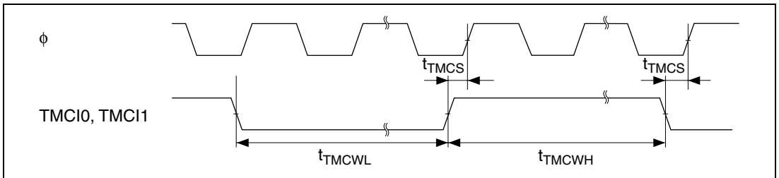
Figure 26.38 8-Bit Timer Clock Input Timing
