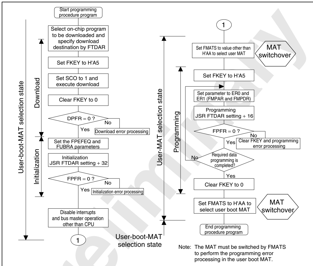
Figure 21.13 Procedure for Programming User MAT in User Boot Mode
