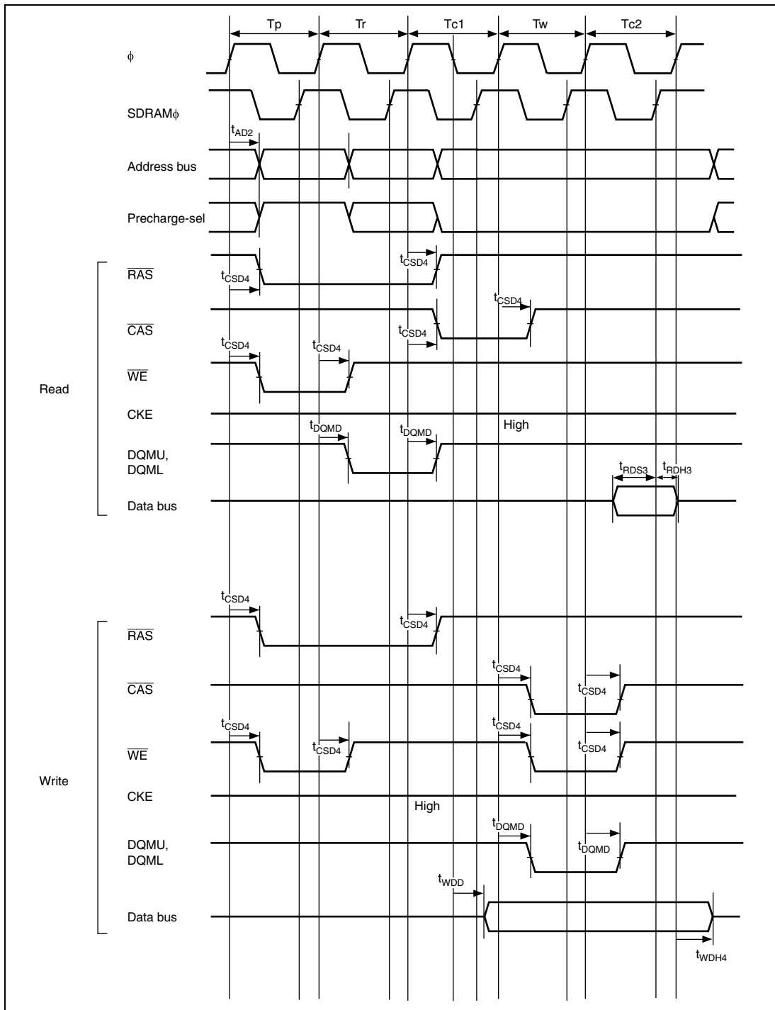
Figure 26.25 Synchronous DRAM Basic Access Timing (CAS Latency 2)
