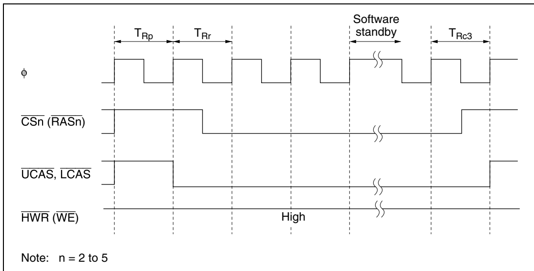
Figure 6.39 Self-Refresh Timing
