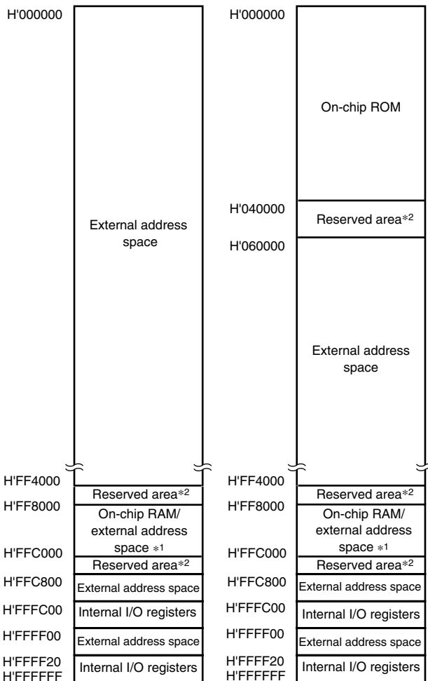
Figure 3.7 Memory Map for H8S/2375 and H8S/2375R (1)
