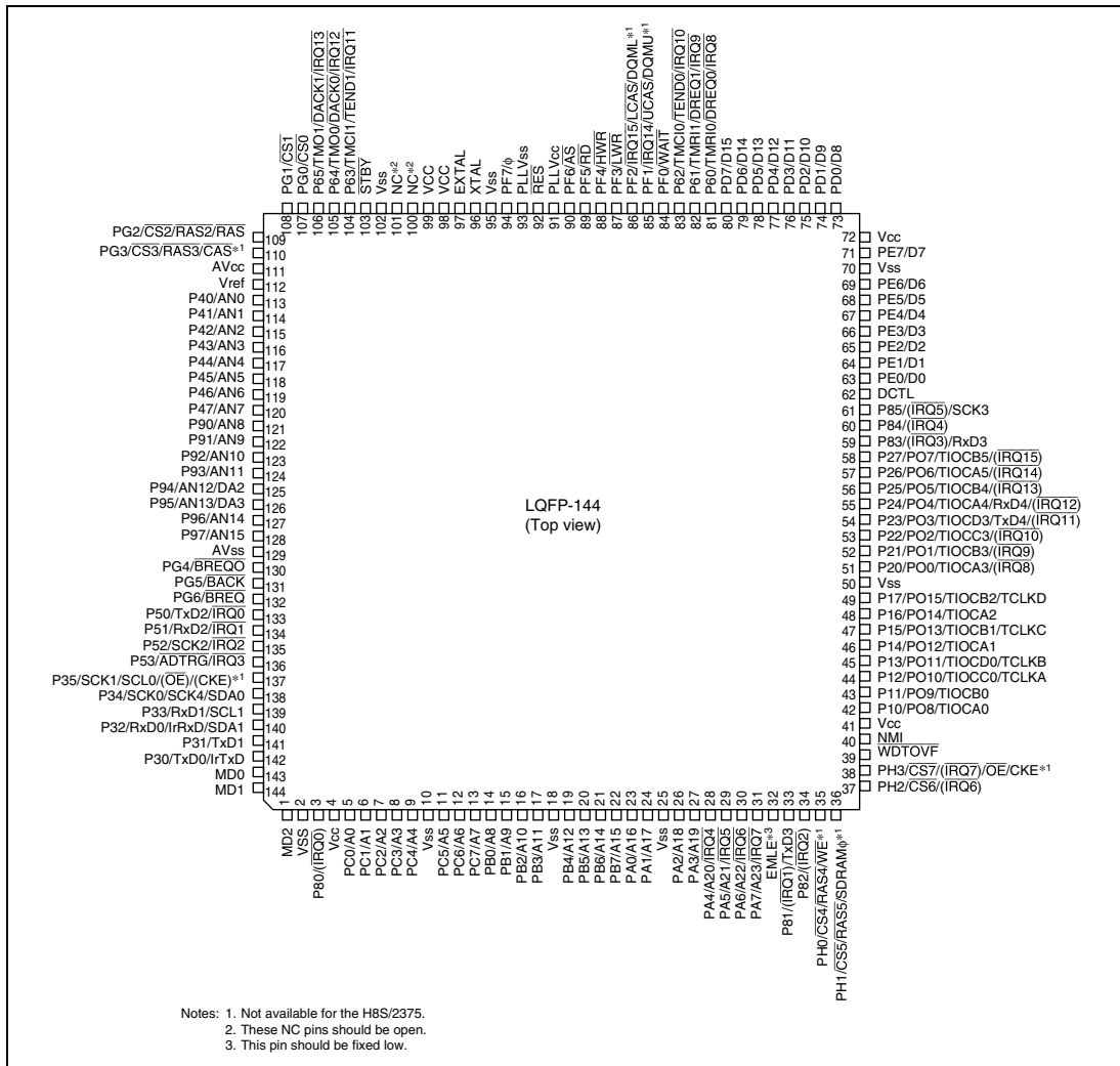
Figure 1.8 Pin Arrangement for H8S2375 and H8S2375R
