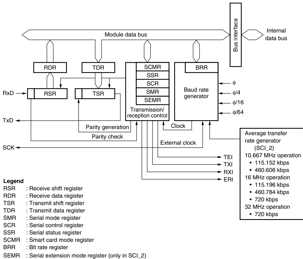
Figure 15.1 Block Diagram of SCI
