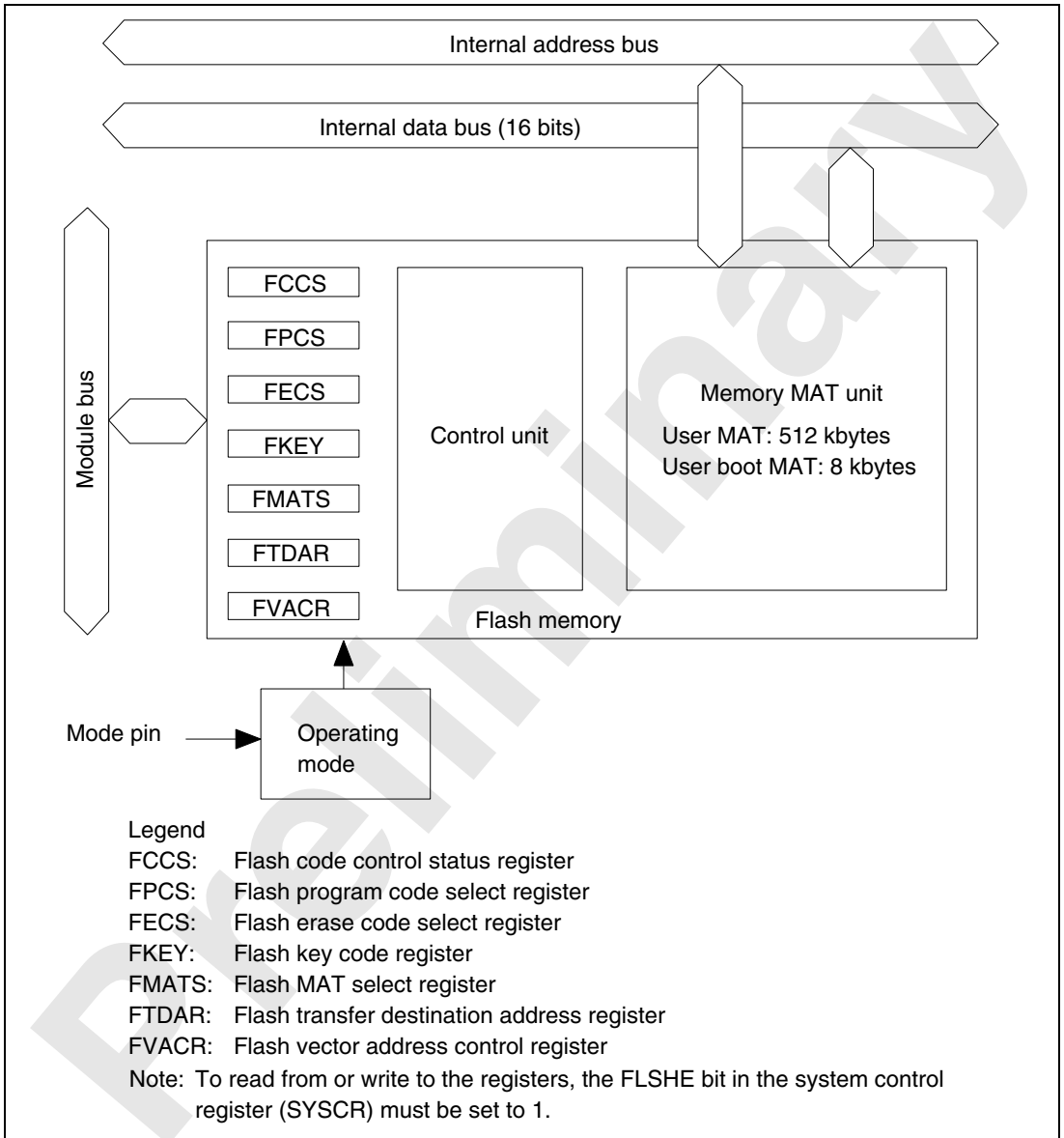
Figure 21.1 Block Diagram of Flash Memory
