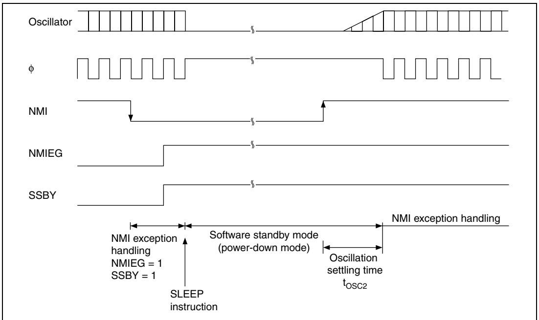
Figure 26.4 (2) Oscillation Settling Timing
