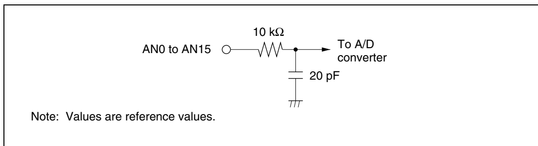
Figure 17.8 Analog Input Pin Equivalent Circuit
