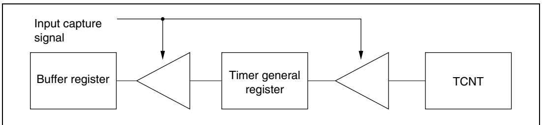
Figure 11.13 Input Capture Buffer Operation
