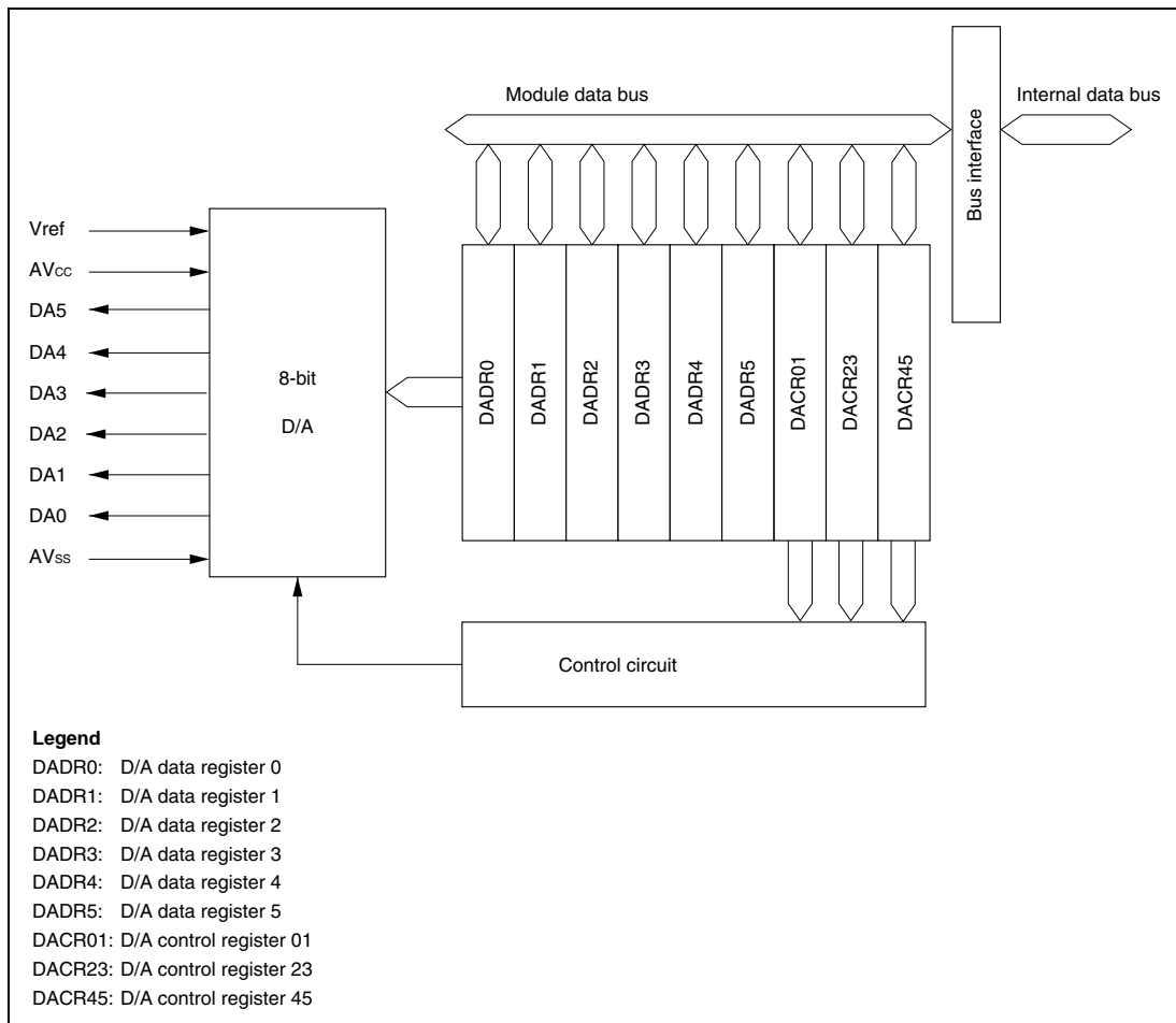
Figure 18.1 Block Diagram of D/A Converter for H8S/2377 and H8S/2377R
