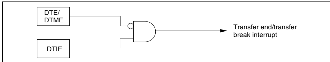
Figure 7.38 Block Diagram of Transfer End/Transfer Break Interrupt
