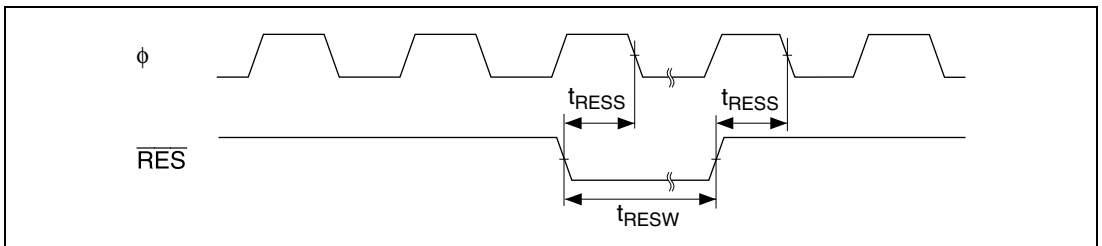
Figure 26.5 Reset Input Timing
