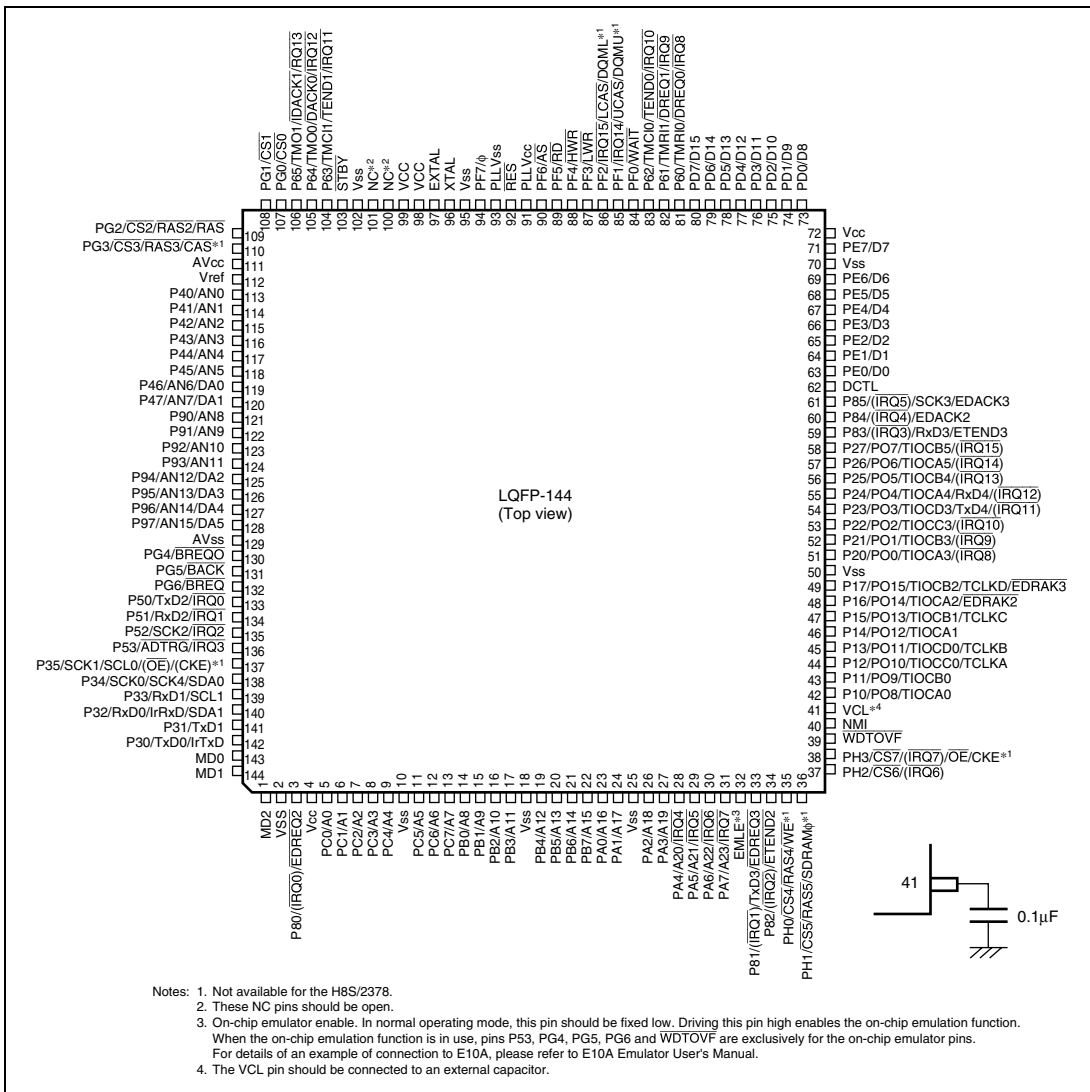
Figure 1.5 Pin Arrangement for H8S2378 and H8S2378R
