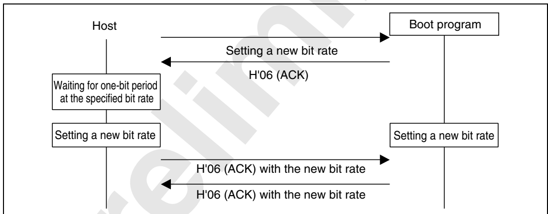
Figure 21.20 New Bit-Rate Selection Sequence
