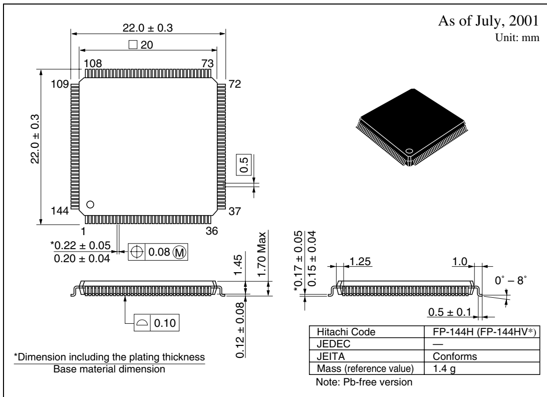
Figure C.1 Package Dimensions (FP-144H)
