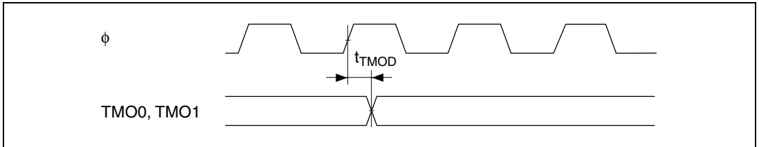
Figure 26.37 8-Bit Timer Output Timing
