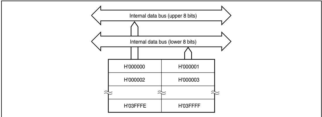
Figure 22.1 Block Diagram of 256-kbyte Masked ROM (HD6432375)
