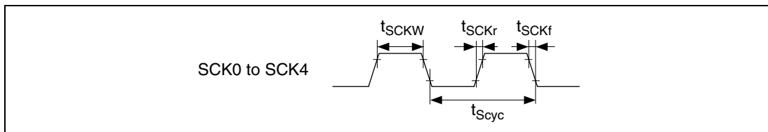
Figure 26.41 SCK Clock Input Timing
