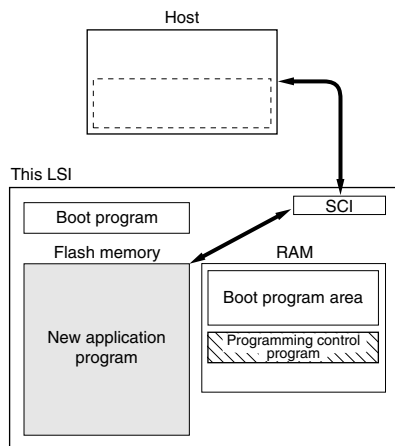
Figure 20.3 Boot Mode
