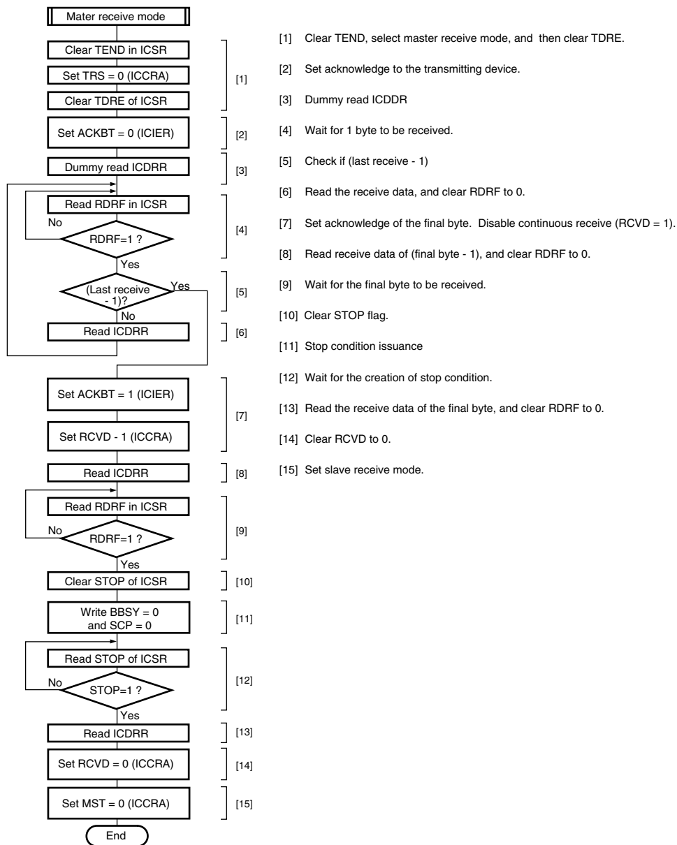
Figure 16.15 Sample Flowchart for Master Receive Mode
