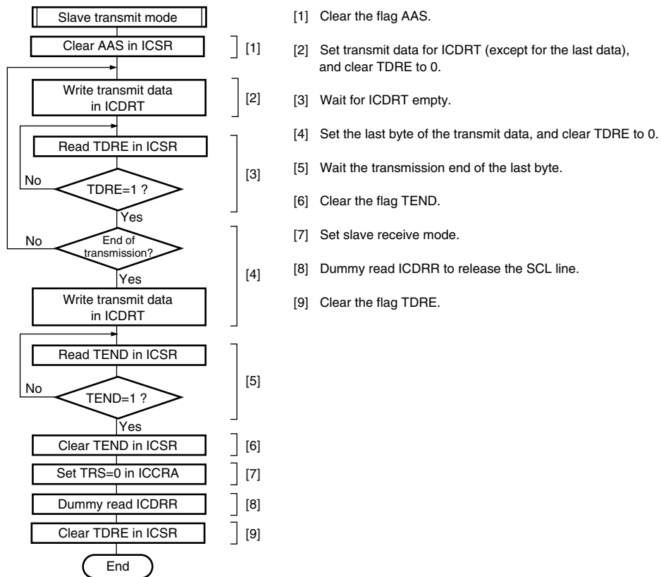
Figure 16.16 Sample Flowchart for Slave Transmit Mode
