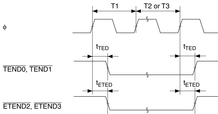
Figure 26.30 DMAC and EXDMAC \overline{\text{TEND}}/\overline{\text{ETEND}} Output Timing
