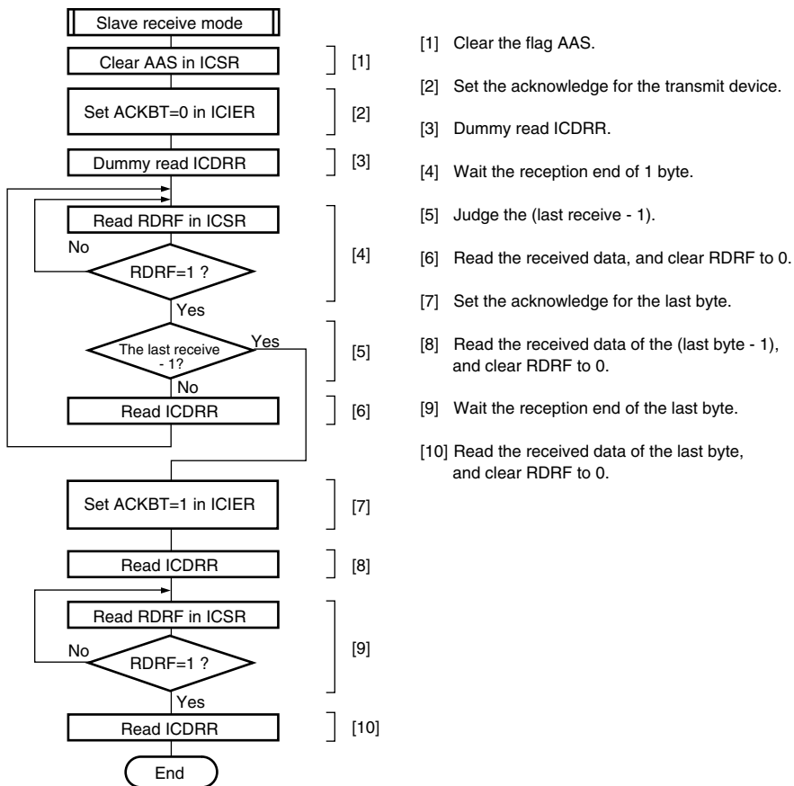
Figure 16.17 Sample Flowchart for Slave Receive Mode
