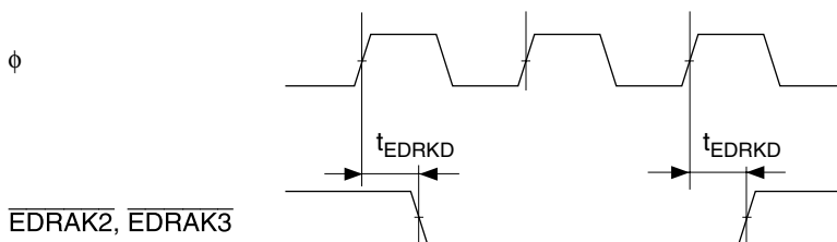
Figure 26.32 EXDMAC \overline{\text{EDRAK}} Output Timing
