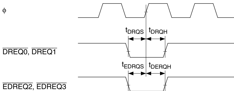
Figure 26.31 DMAC and EXDMAC \overline{\text{DREQ}}/\overline{\text{EDREQ}} Input Timing
