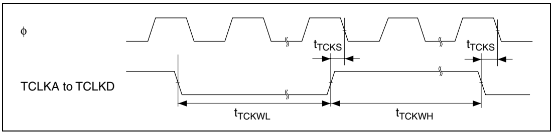
Figure 26.36 TPU Clock Input Timing
