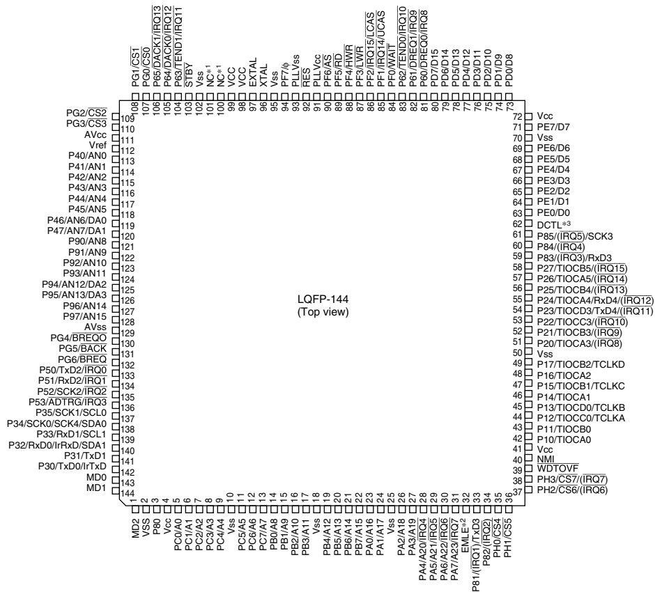
Figure 1.7 Pin Arrangement for H8S2376
