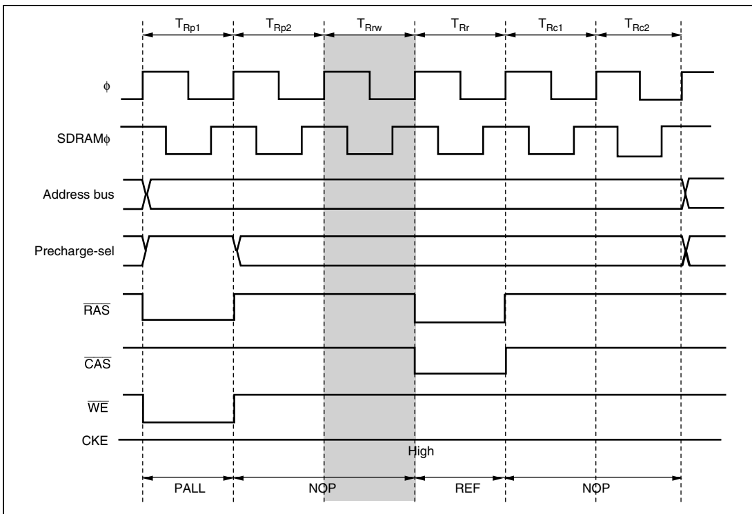
Figure 6.55 Auto Refresh Timing (TPC = 1, TPC0 = 1, RCW1 = 0, RCW0 = 1)
