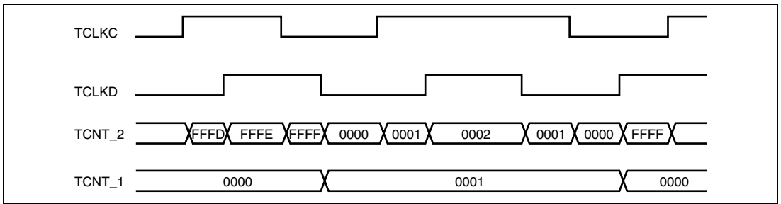
Figure 11.19 Example of Cascaded Operation (2)
