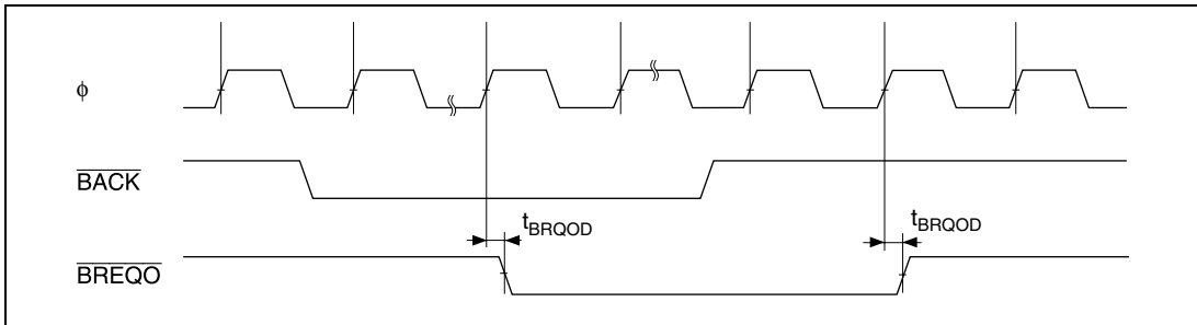
Figure 26.24 External Bus Request Output Timing
