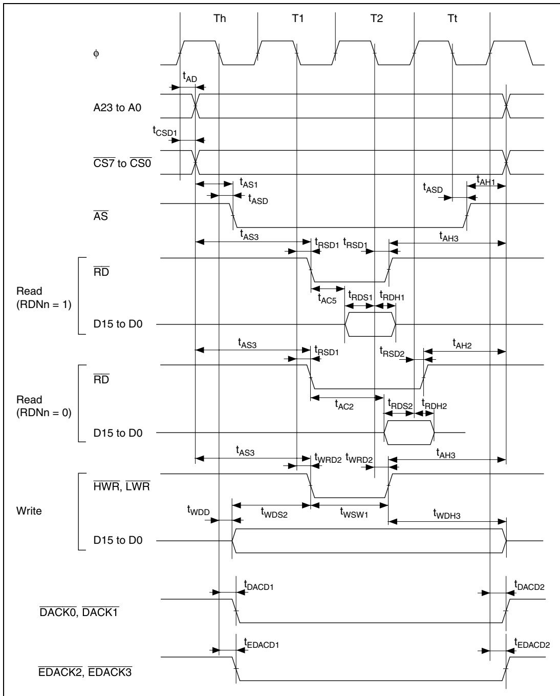
Figure 26.10 Basic Bus Timing: Two-State Access ( \overline{\text{CS}} Assertion Period Extended)
