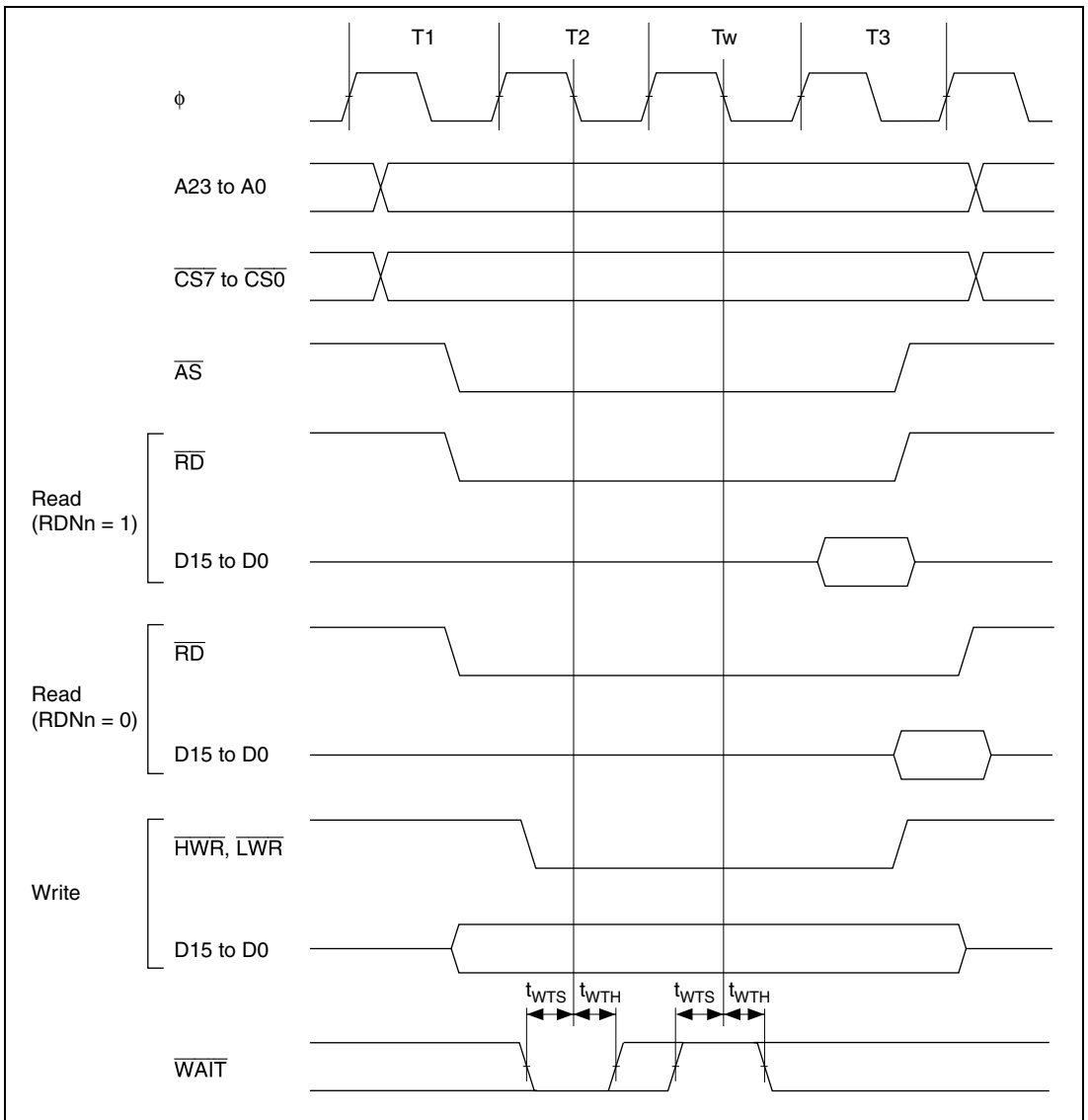
Figure 26.9 Basic Bus Timing: Three-State Access, One Wait
