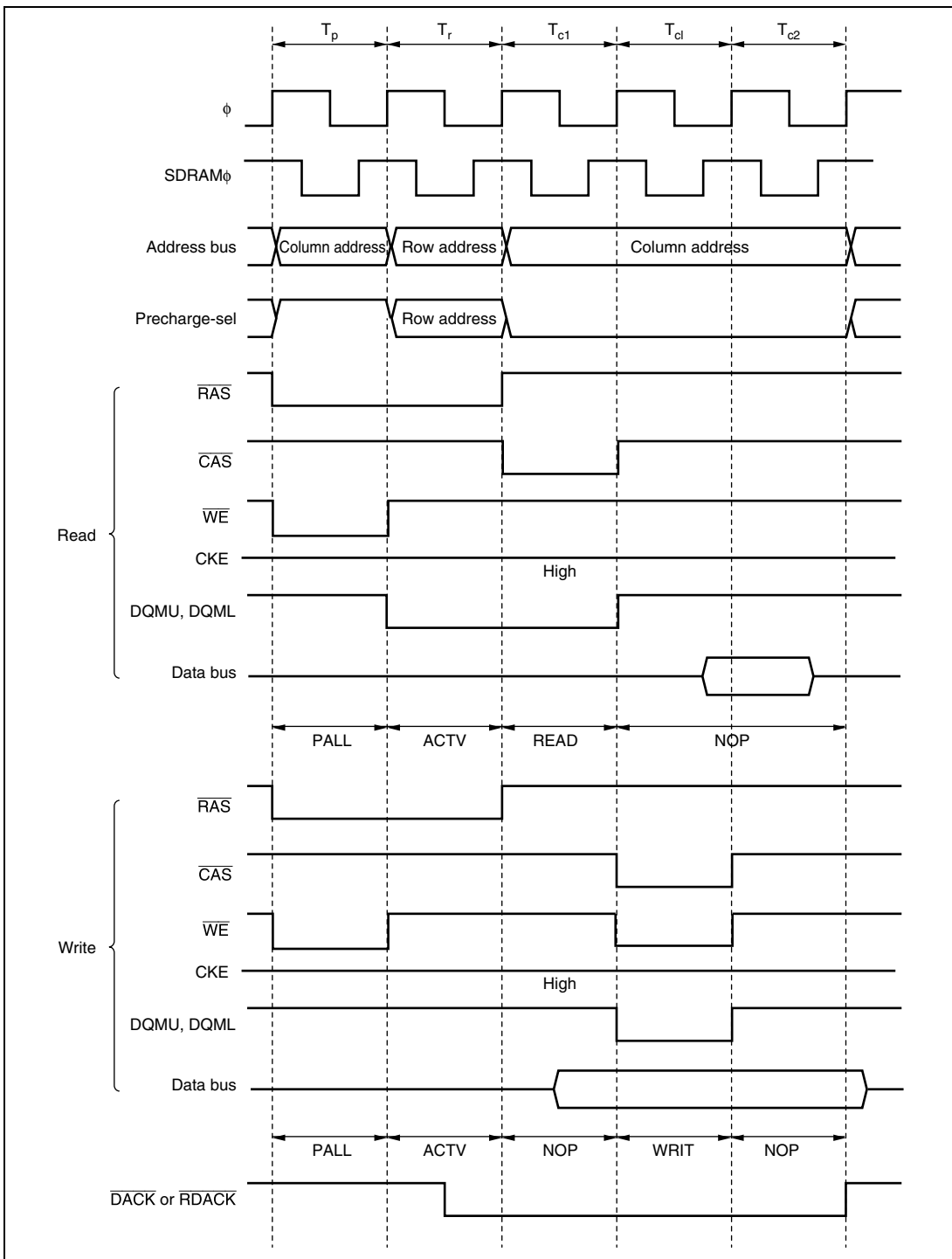
Figure 6.61 Example of \overline{DACK}/\overline{EDACK} Output Timing when DDS = 0 or EDDS = 0
