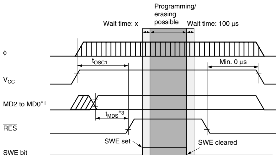
(1) Boot Mode
