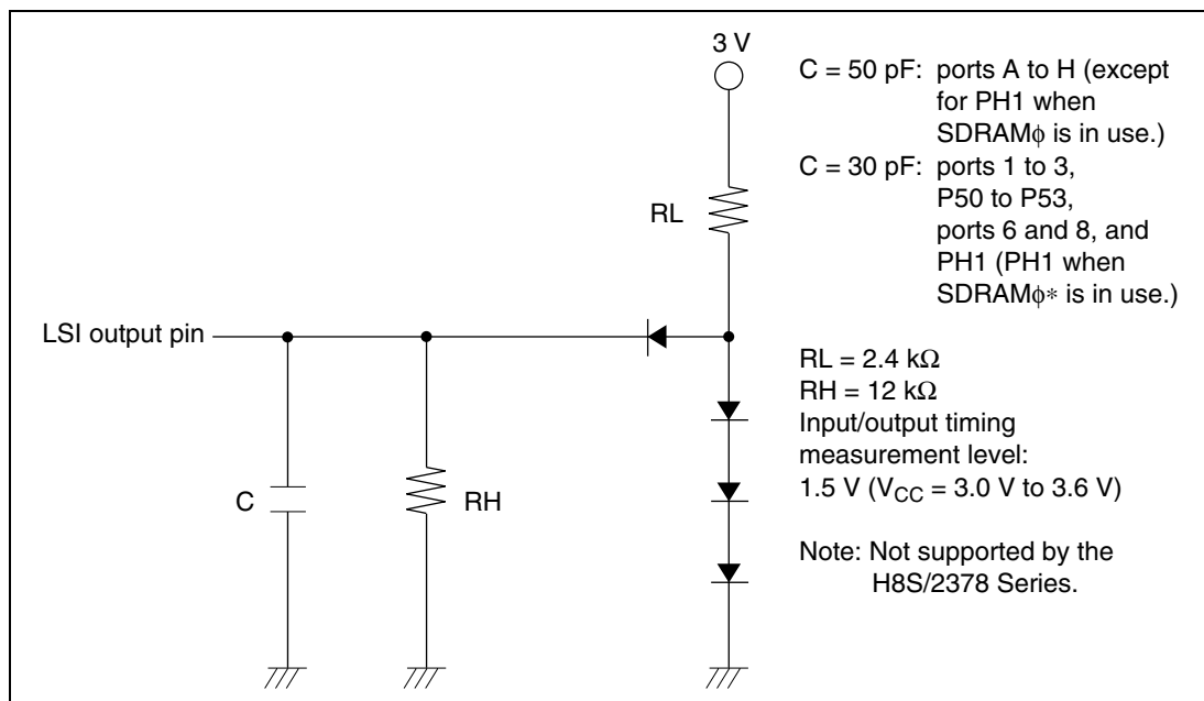
Figure 26.1 Output Load Circuit
