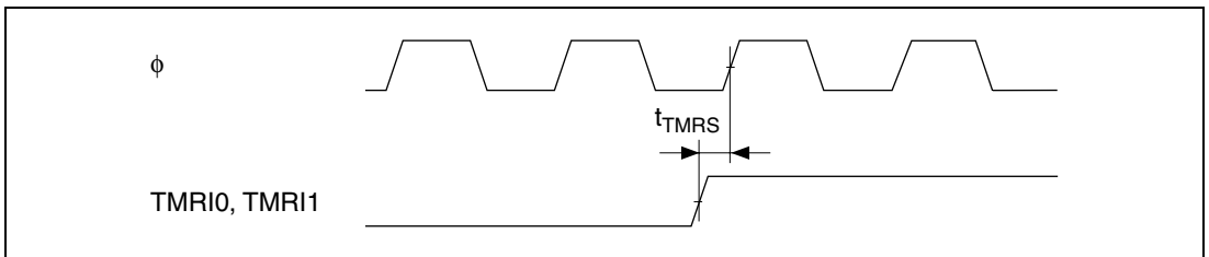
Figure 26.39 8-Bit Timer Reset Input Timing
