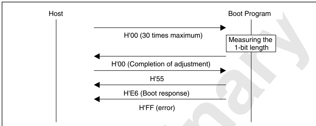
Figure 21.18 Bit-Rate-Adjustment Sequence
