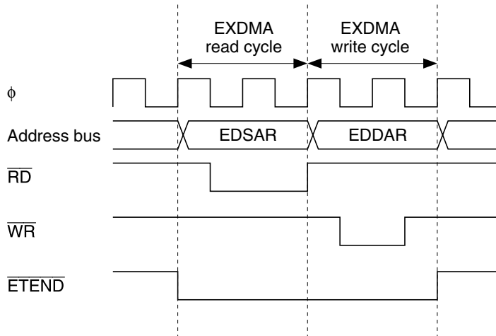
Figure 8.2 Example of Timing in Dual Address Mode
