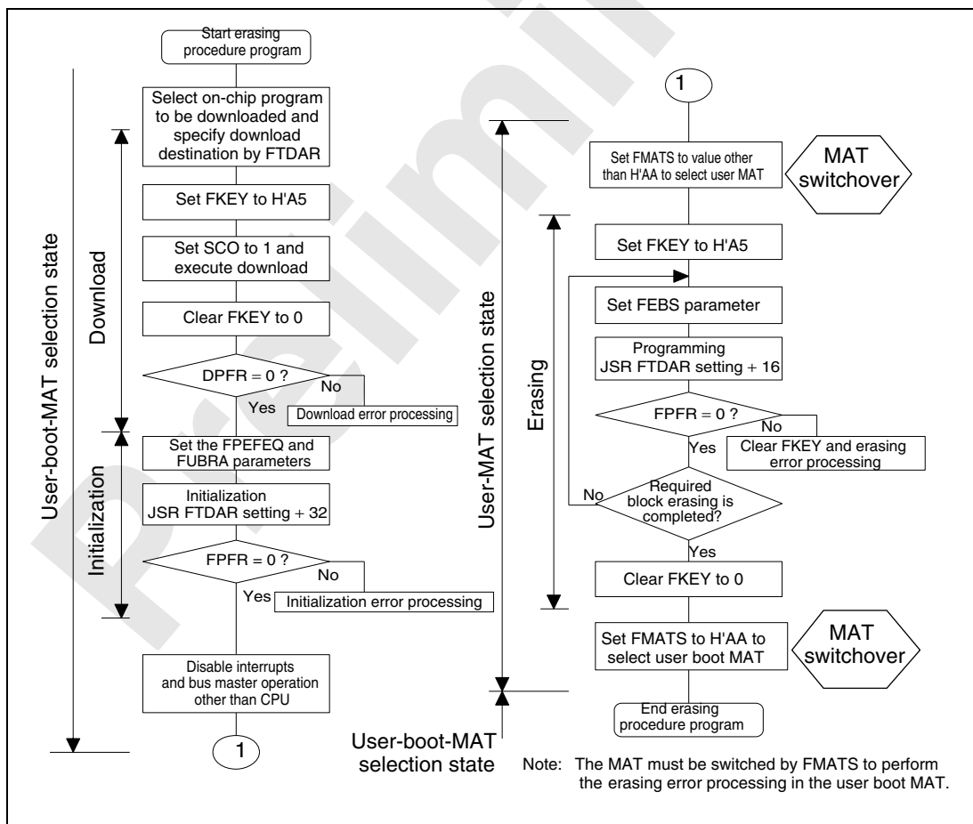
Figure 21.14 Procedure for Erasing User MAT in User Boot Mode
