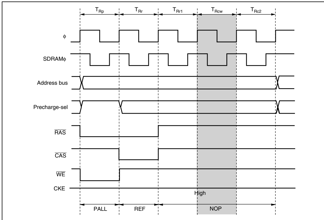
Figure 6.56 Auto Refresh Timing (TPC = 0, TPC0 = 0, RLW1 = 0, RLW0 = 1)
