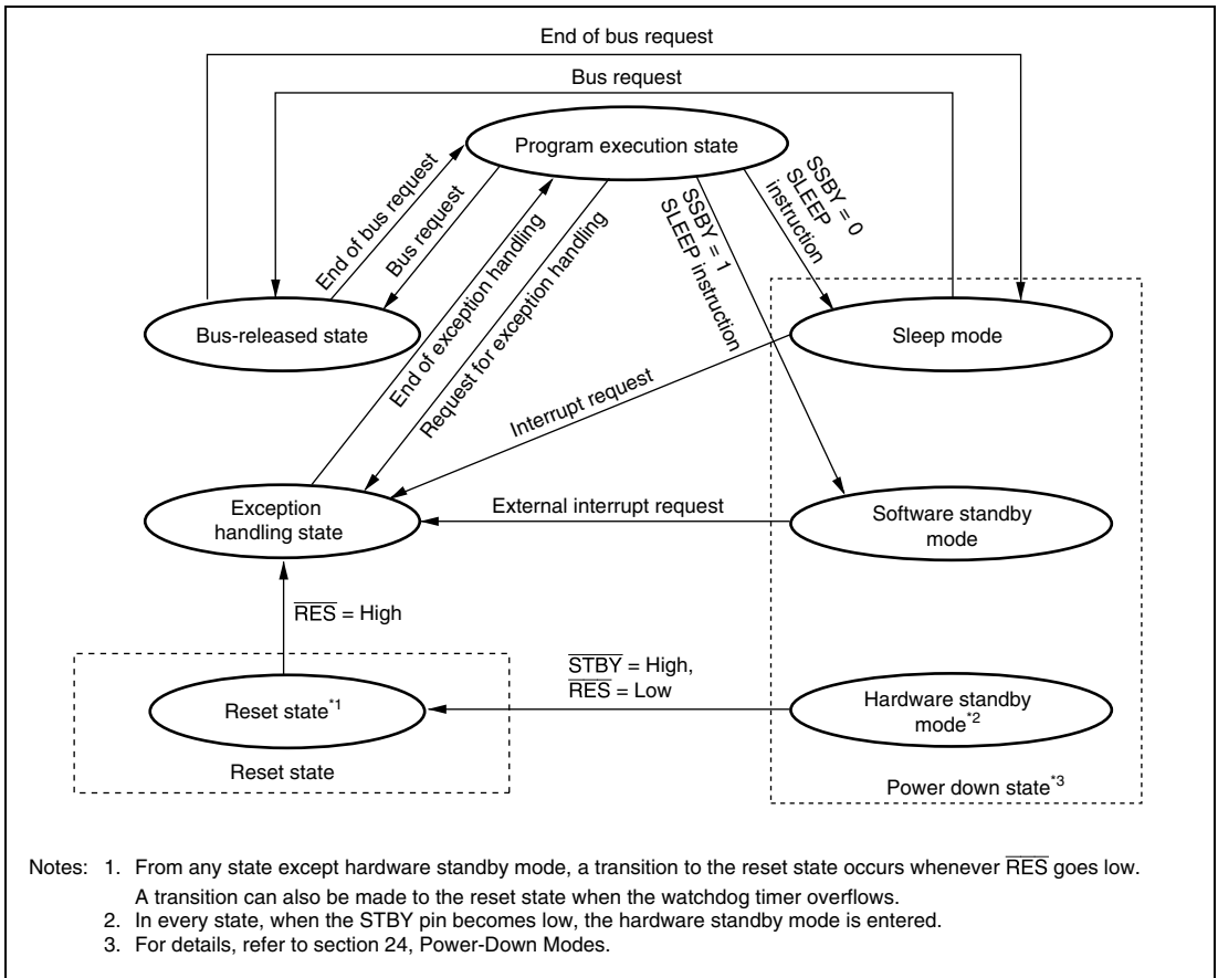
Figure 2.13 State Transitions
