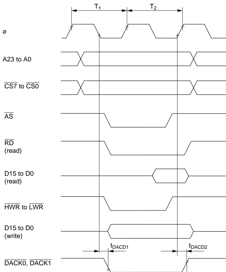
Figure 25-16 DMAC Single Address Transfer Timing / Two-State Access
