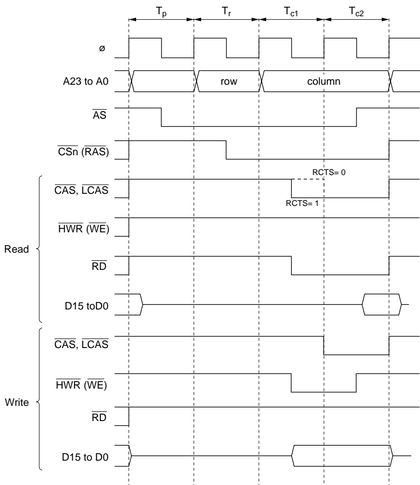
Figure 7-15 Basic Access Timing
