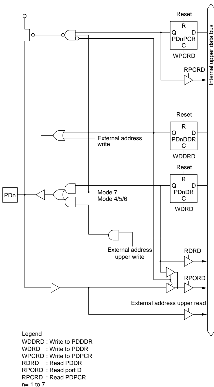
Figure C-12 Port D Block Diagram (Pin PDn)
