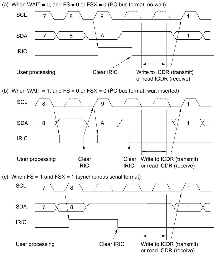
Figure 18-12 IRIC Setting Timing and SCL Control
