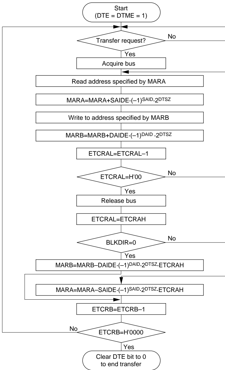
Figure 8-15 Operation Flow in Block Transfer Mode
