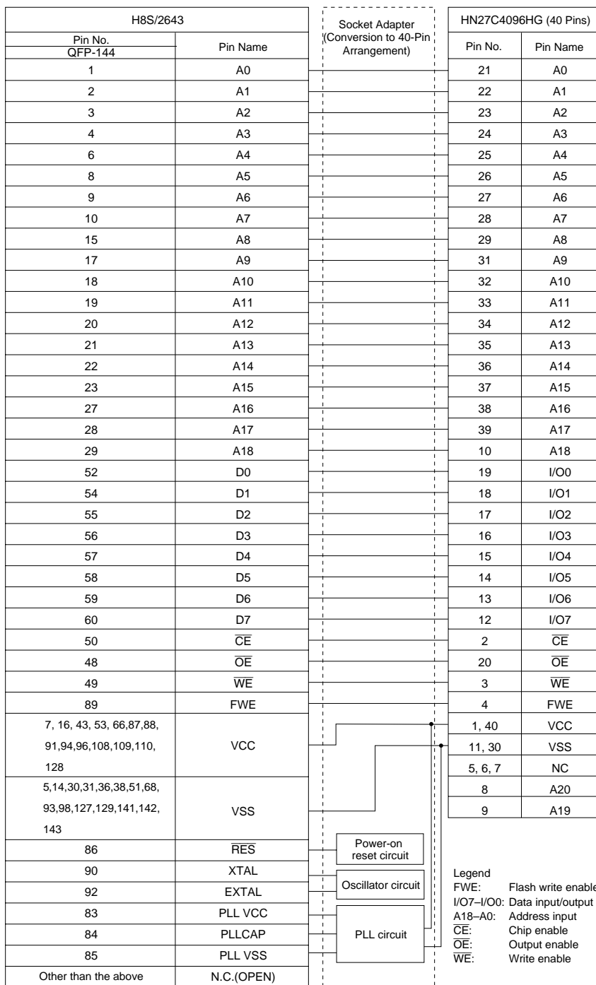
Figure 22-19 Socket Adapter Pin Correspondence Diagram
