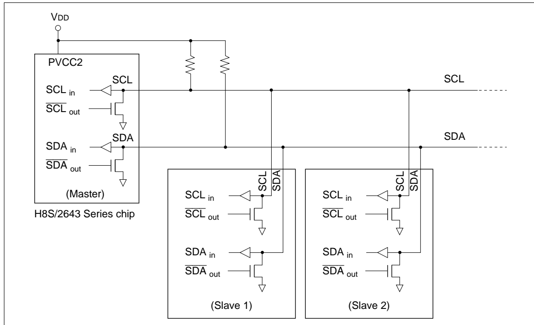
Figure 18-2 I²C Bus Interface Connections (Example: H8S/2643 Series Chip as Master)
