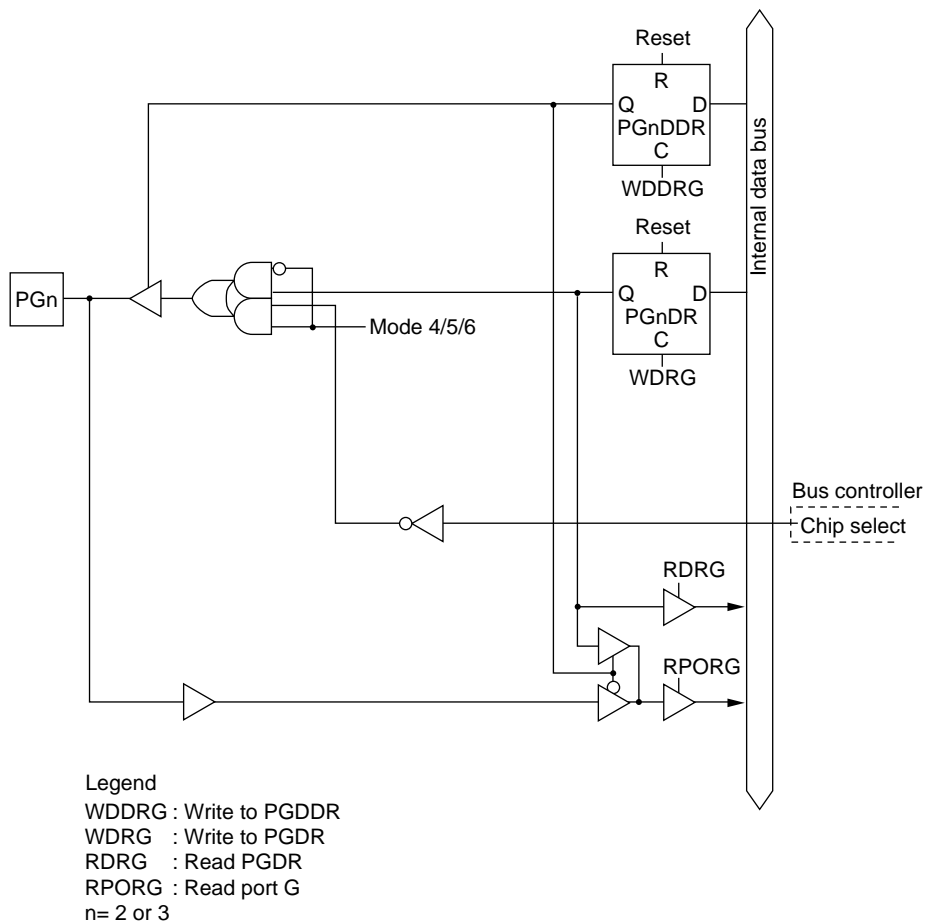
Figure C-15 (c) Port G Block Diagram (Pins PG2 and PG3)
