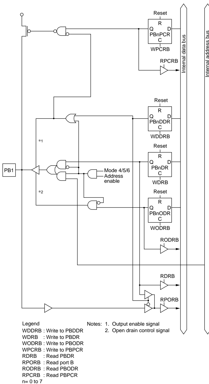
Figure C-10 Port B Block Diagram (Pins PB0 to PB7)
