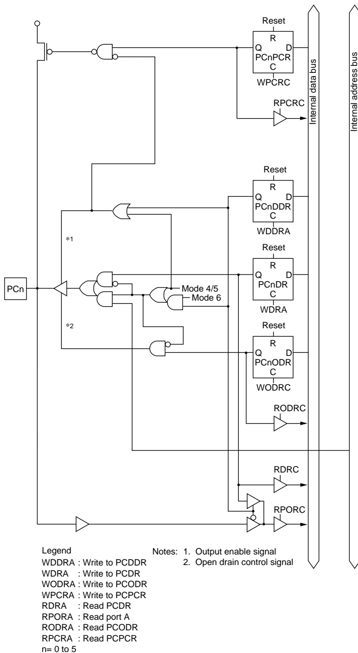
Figure C-11 (a) Port C Block Diagram (Pins PC0 to PC5)
