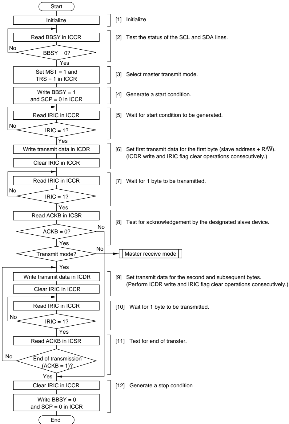
Figure 18-14 Flowchart for Master Transmit Mode (Example)
