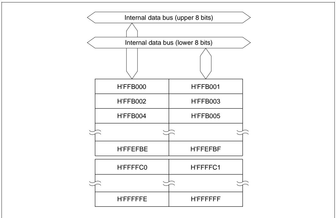
Figure 21-1 Block Diagram of RAM (H8S/2643 Series)
