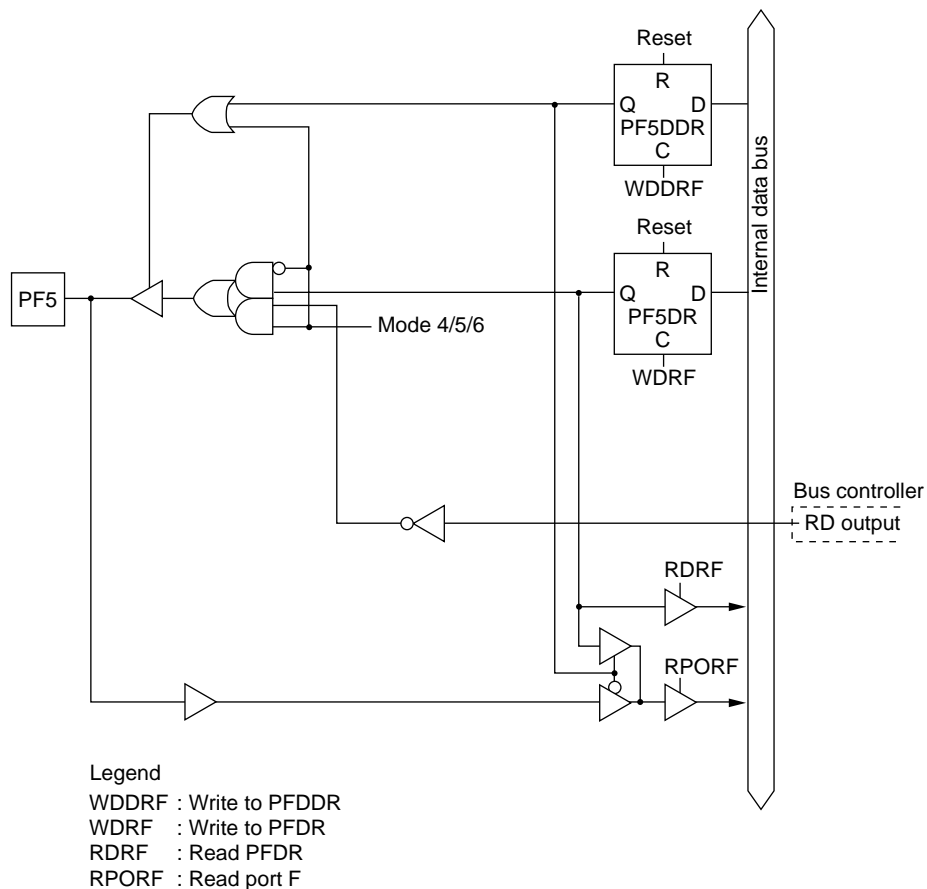
Figure C-14 (f) Port F Block Diagram (Pin PF5)
