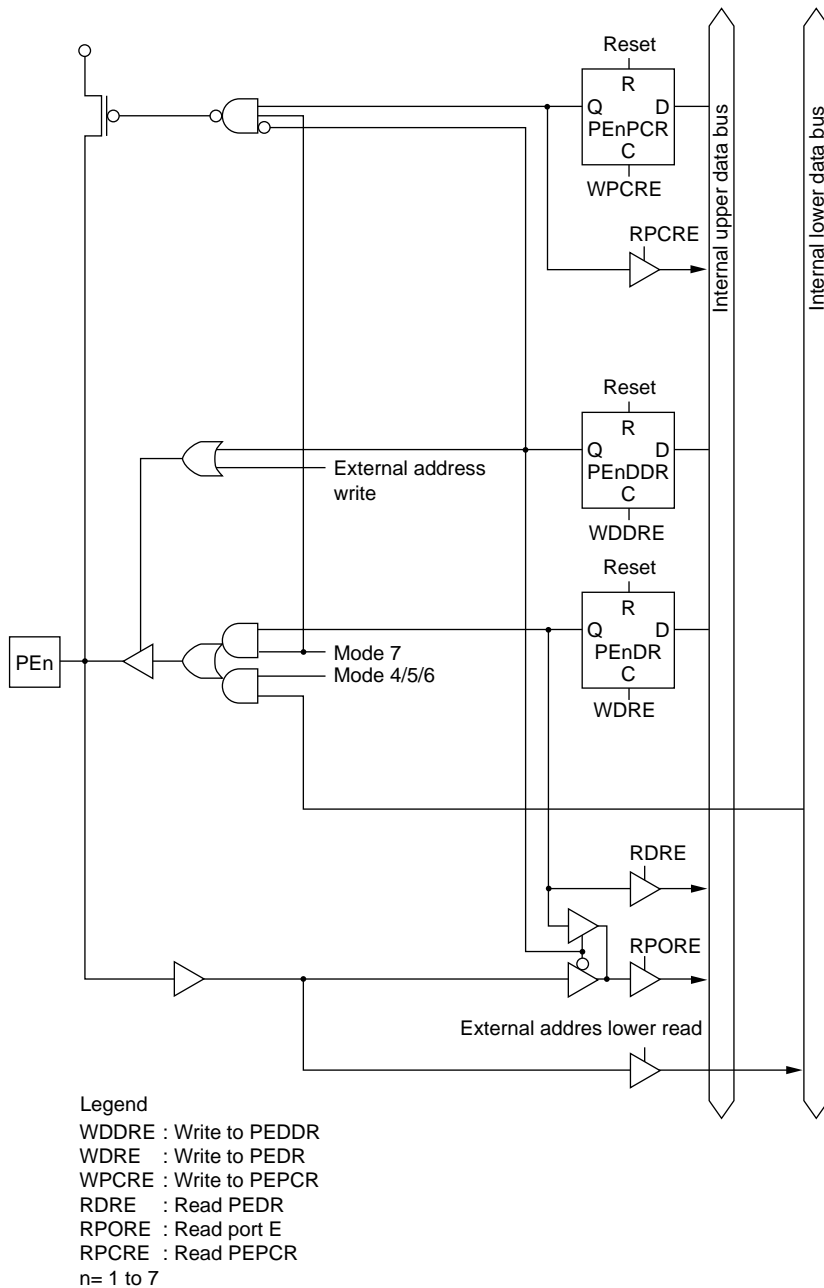
Figure C-13 Port E Block Diagram (Pin PEn)
