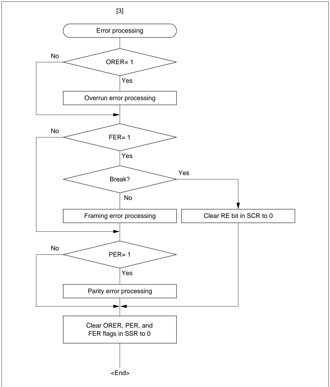
Figure 16-7 Sample Serial Reception Data Flowchart (cont)
