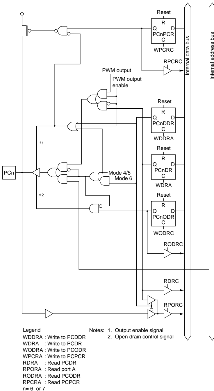
Figure C-11 (b) Port C Block Diagram (Pins PC6 and PC7)
