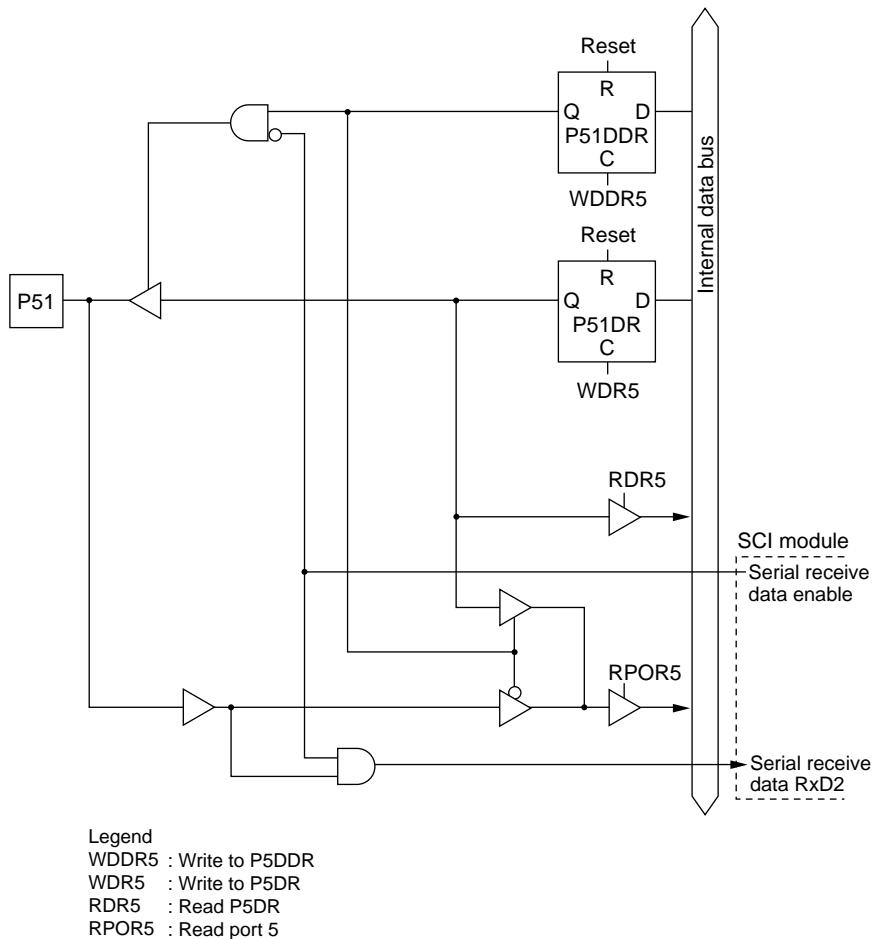
Figure C-5 (b) Port 5 Block Diagram (Pin P51)
