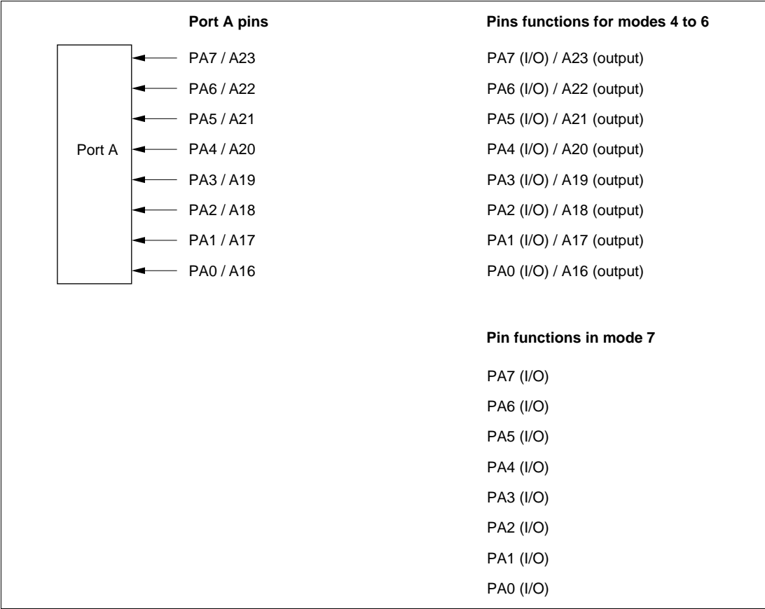
Figure 10-9 Port A Pin Functions
