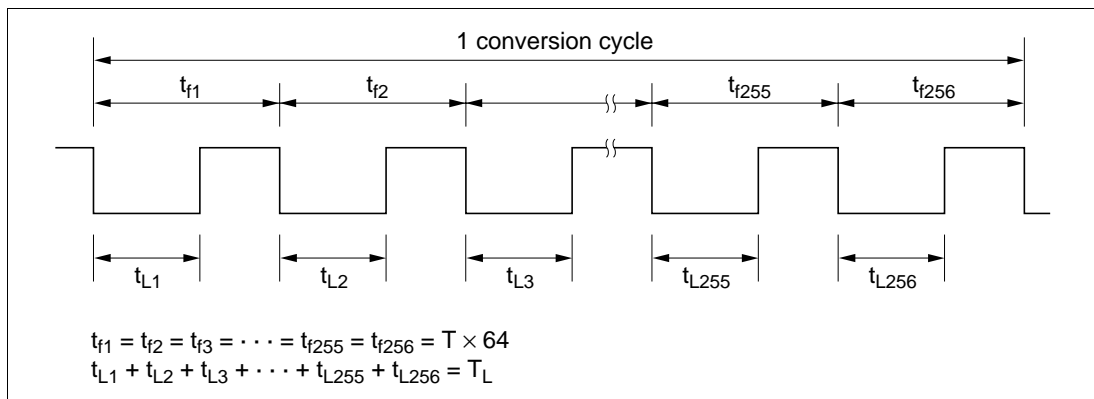
Figure 14-4 (1) Output Waveform
