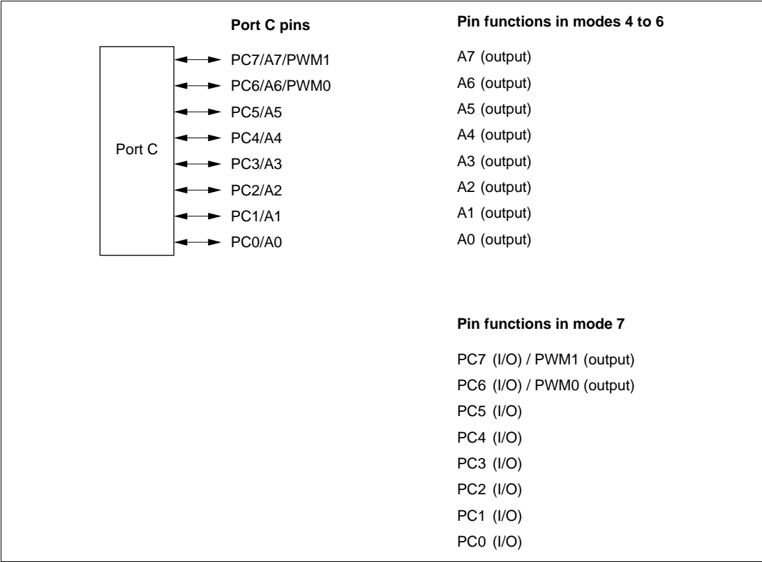
Figure 10-15 Port C Pin Functions
