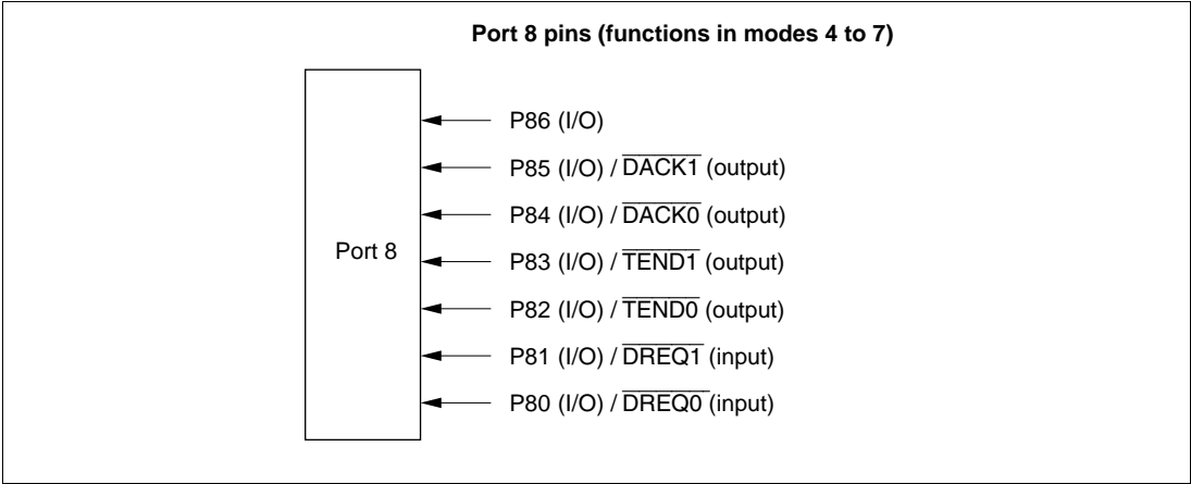
Figure 10-7 Port 8 Pin Functions
