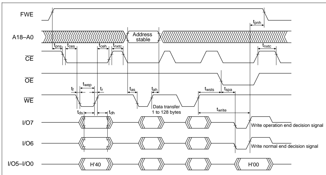
Figure 22-24 Auto-Program Mode Timing Waveforms
