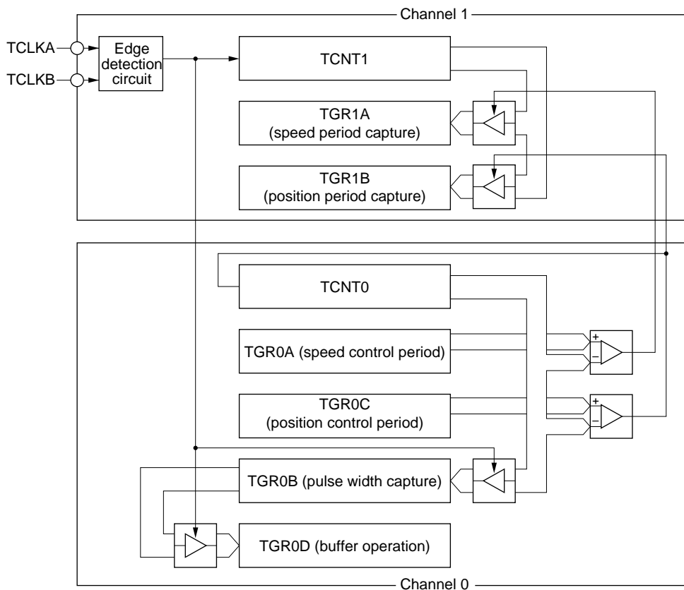
Figure 11-33 Phase Counting Mode Application Example
