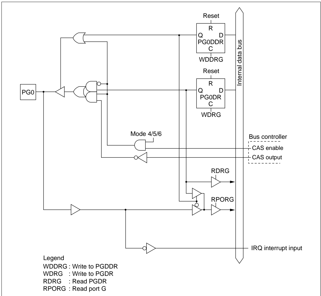
Figure C-15 (a) Port G Block Diagram (Pin PG0)
