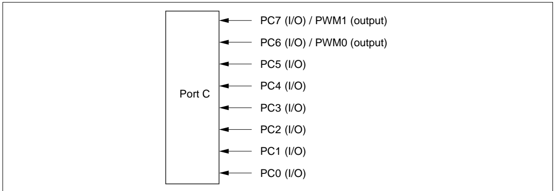
Figure 10-18 Port C Pin Functions (Mode 7)
