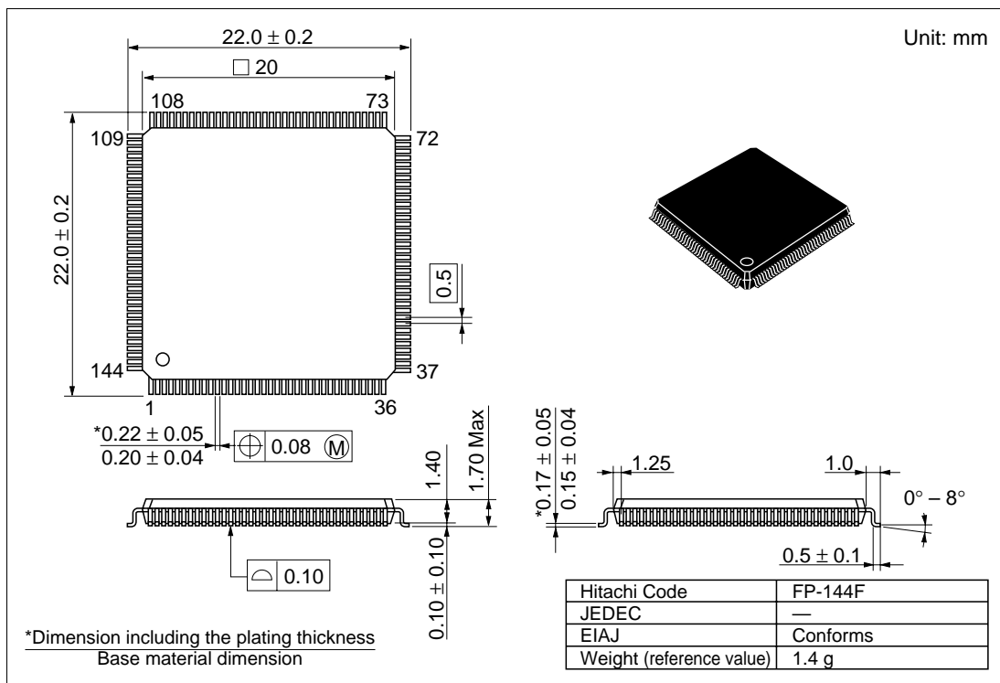
Figure G-1 FP-144F Package Dimensions
