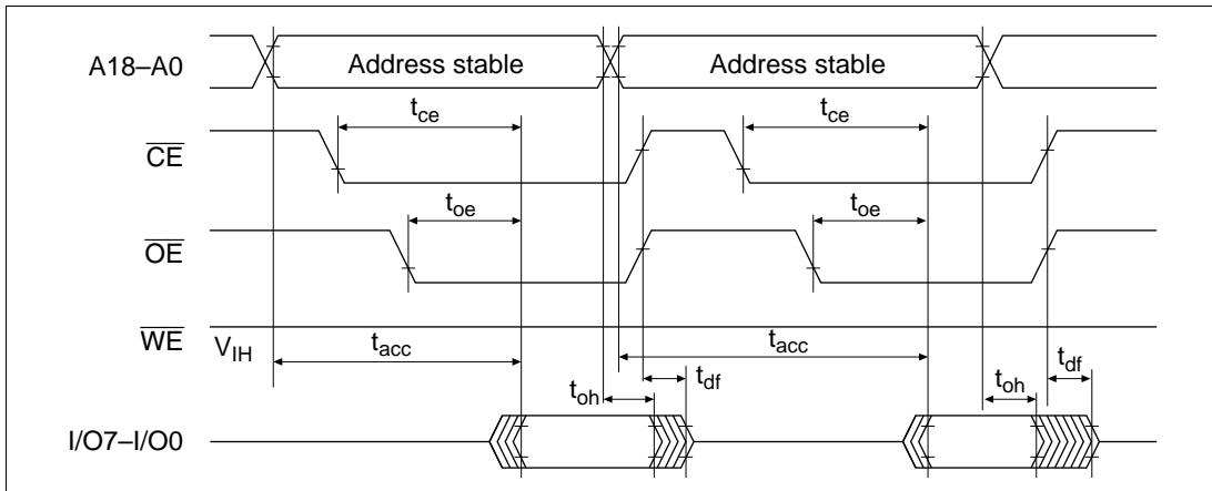
Figure 22-23 \overline{CE} and \overline{OE} Clock System Read Timing Waveforms
