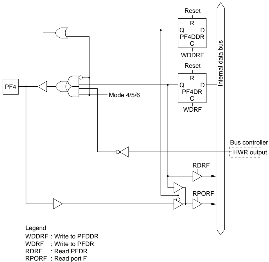
Figure C-14 (e) Port F Block Diagram (Pin PF4)
