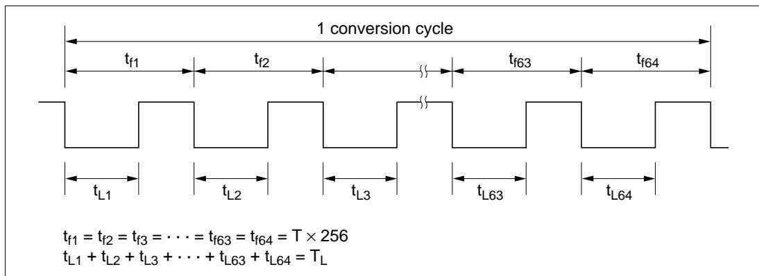
Figure 14-4 (2) Output Waveform
