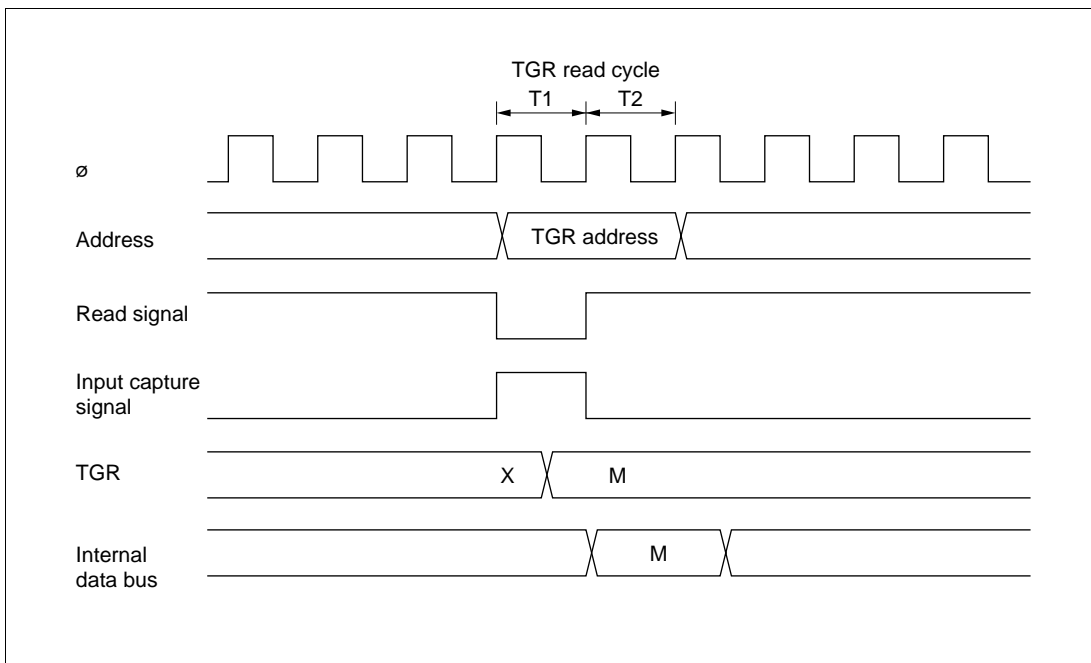
Figure 11-53 Contention between TGR Read and Input Capture
