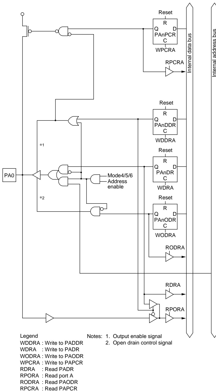
Figure C-9 (a) Port A Block Diagram (Pin PA0)
