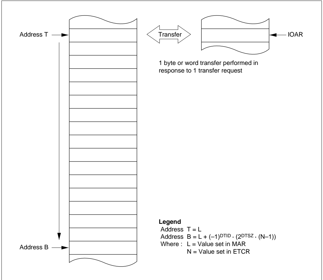
Figure 8-3 Operation in Sequential Mode
