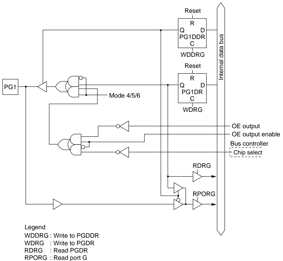
Figure C-15 (b) Port G Block Diagram (Pin PG1)
