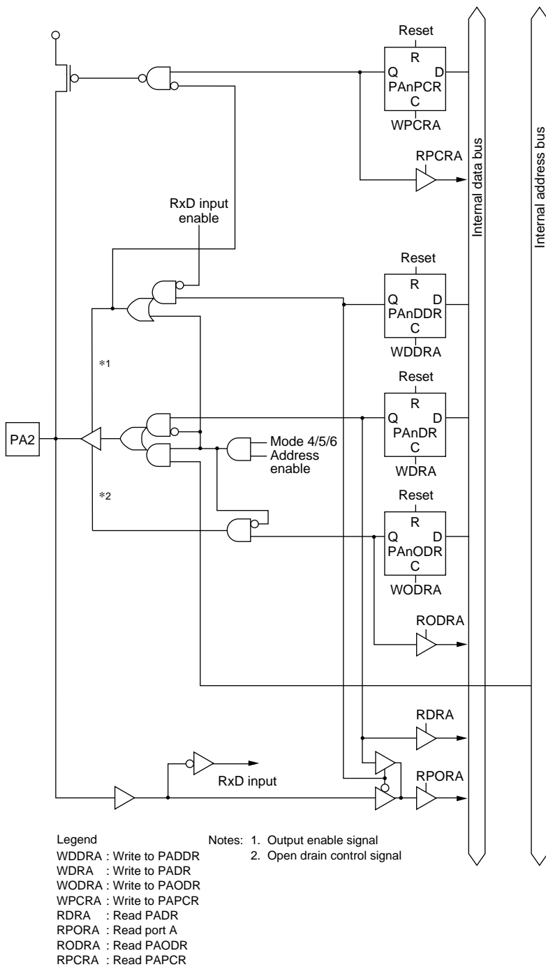
Figure C-9 (c) Port A Block Diagram (Pin PA2)
