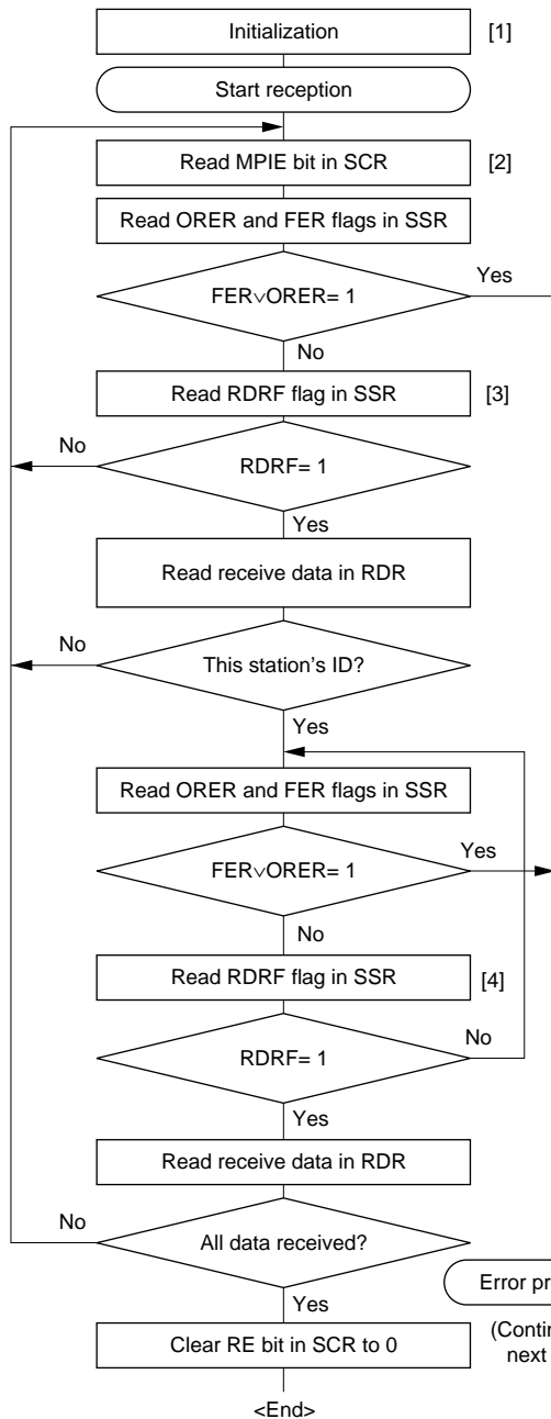
Figure 16-12 Sample Multiprocessor Serial Reception Flowchart
