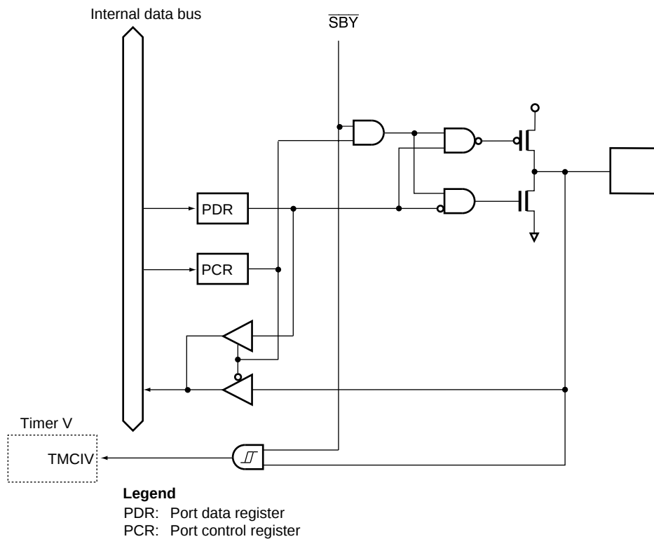
Figure B.12 Port 7 Block Diagram (P75)
