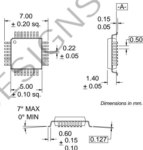
Package Style: LQFP-32
