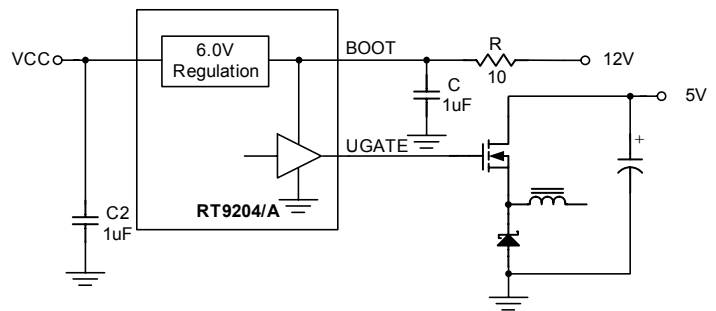
Fig.4 Dual Power Supply Operation
