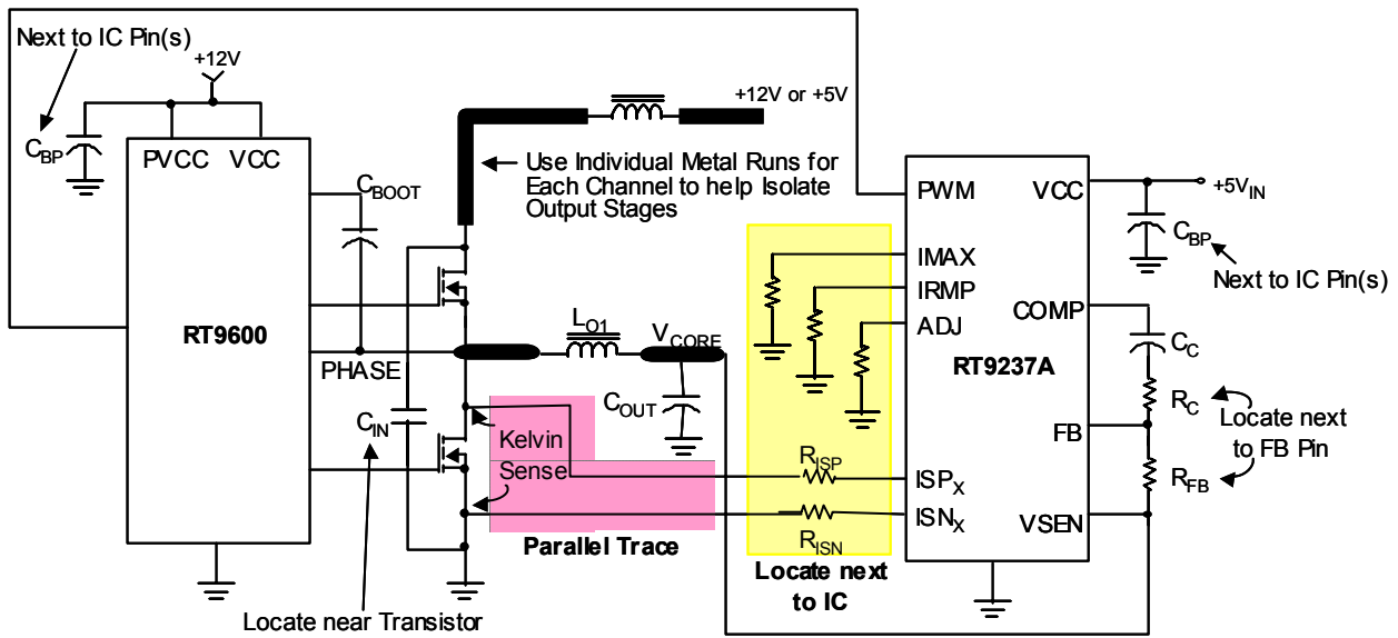
Fig.8 Layout Consideration
