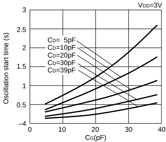
10.9 Oscillation Start Time vs. CG
