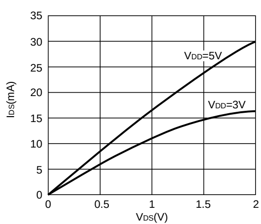
10.10 Nch Open Drain Output Ibs vs. Vbs
