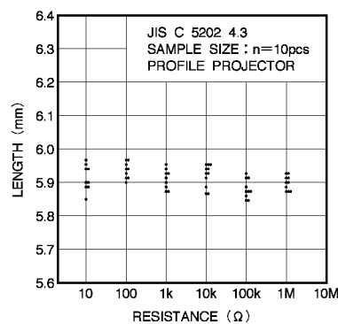
Fig.4 Dimensions (length)
