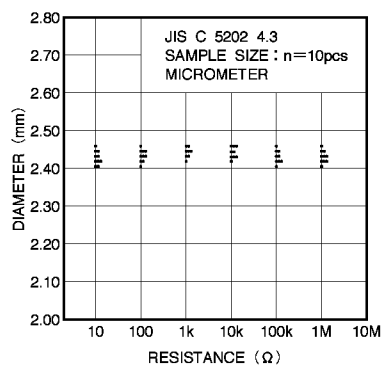
Fig.3 Dimensions (diameter)
