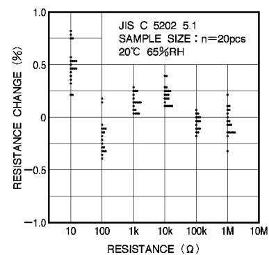
Fig.5 DC resistance
