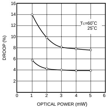
Fig. 8 Dependence of droop on output
