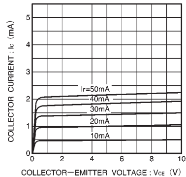
Fig.9 Output characteristics
