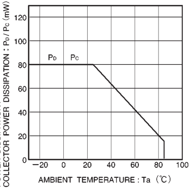
Fig.1 Power dissipation and collector power dissipation vs. ambient temperature
