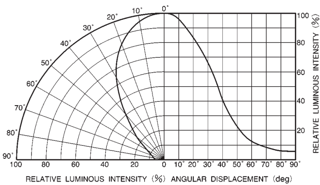
Fig.8 Directional pattern
