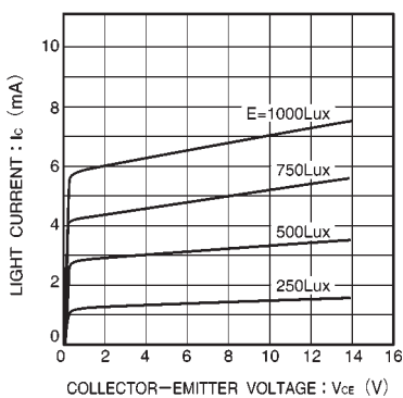
Fig.4 Output characteristics
