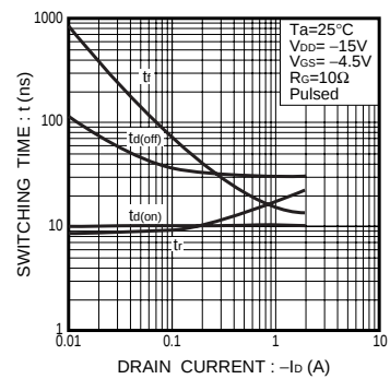
Fig.9 Switching Characteristics
