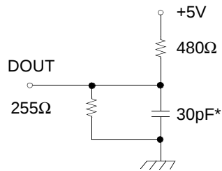
Output Loads(A)
