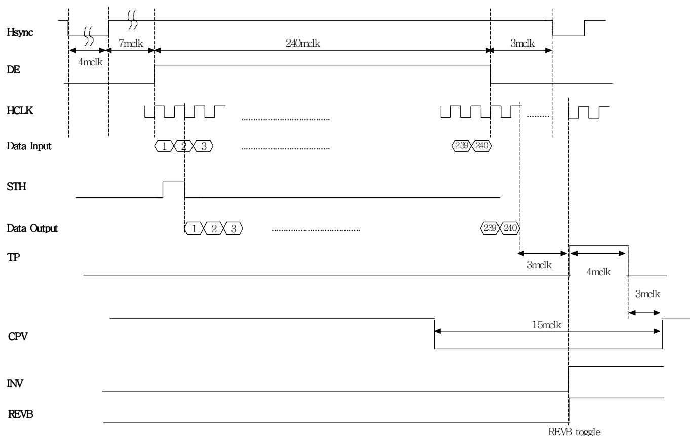
Horizontal Timing Chart
