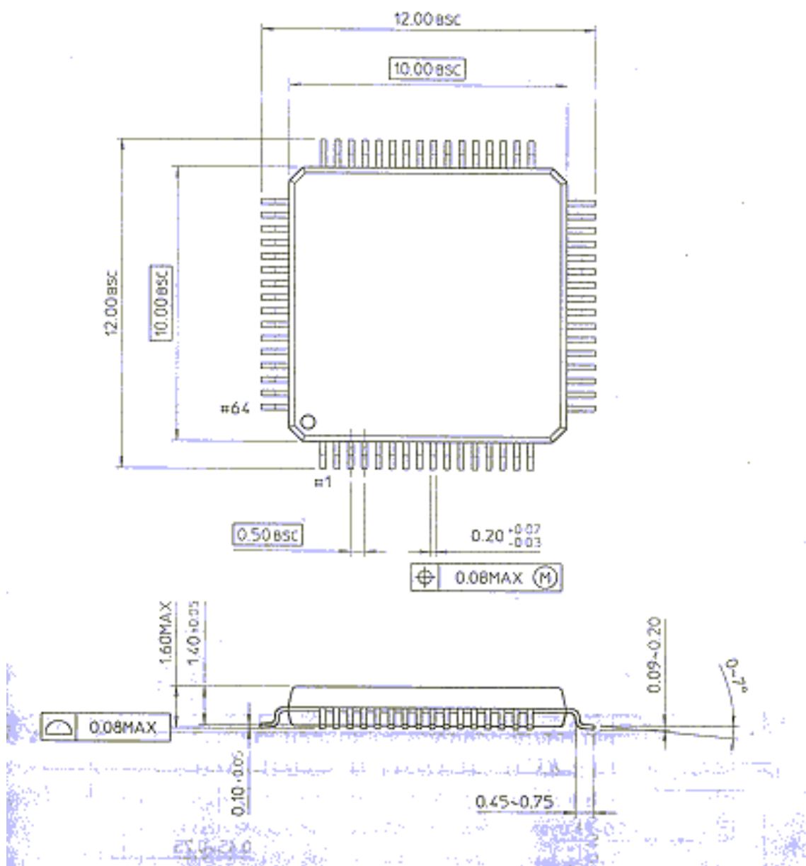
Fig.3 Dimension
