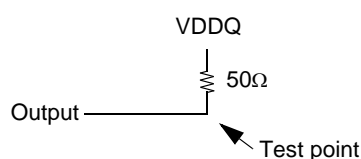
Figure 2 : Pulldown slew rate test load
