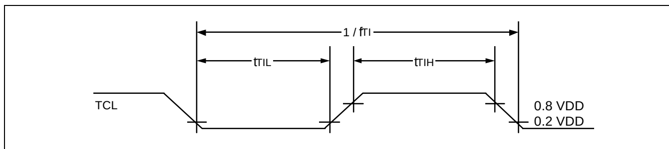
Figure 14-6. TCL Timing
