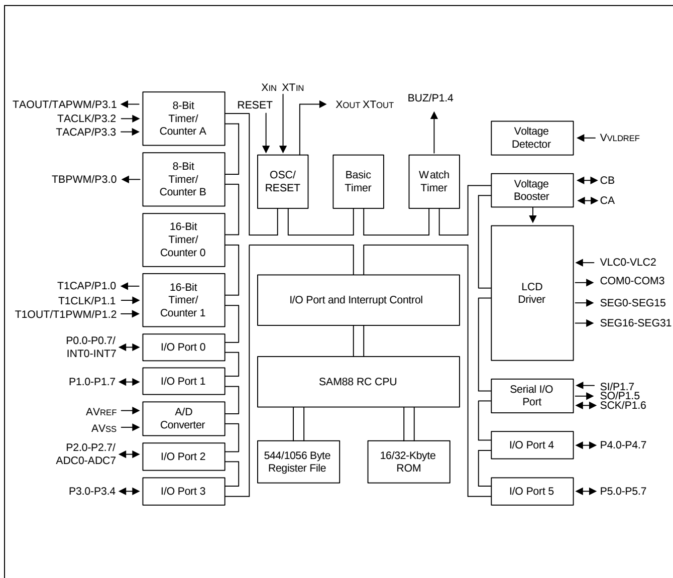
Figure 1-1. Block Diagram
