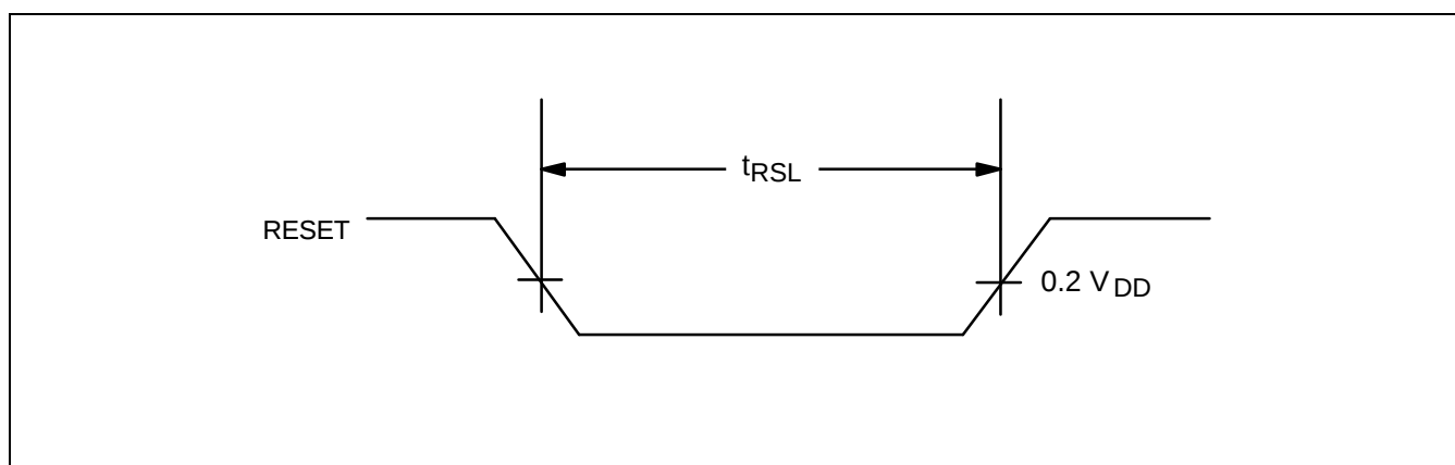
Figure 19-2. Input Timing for RESET
