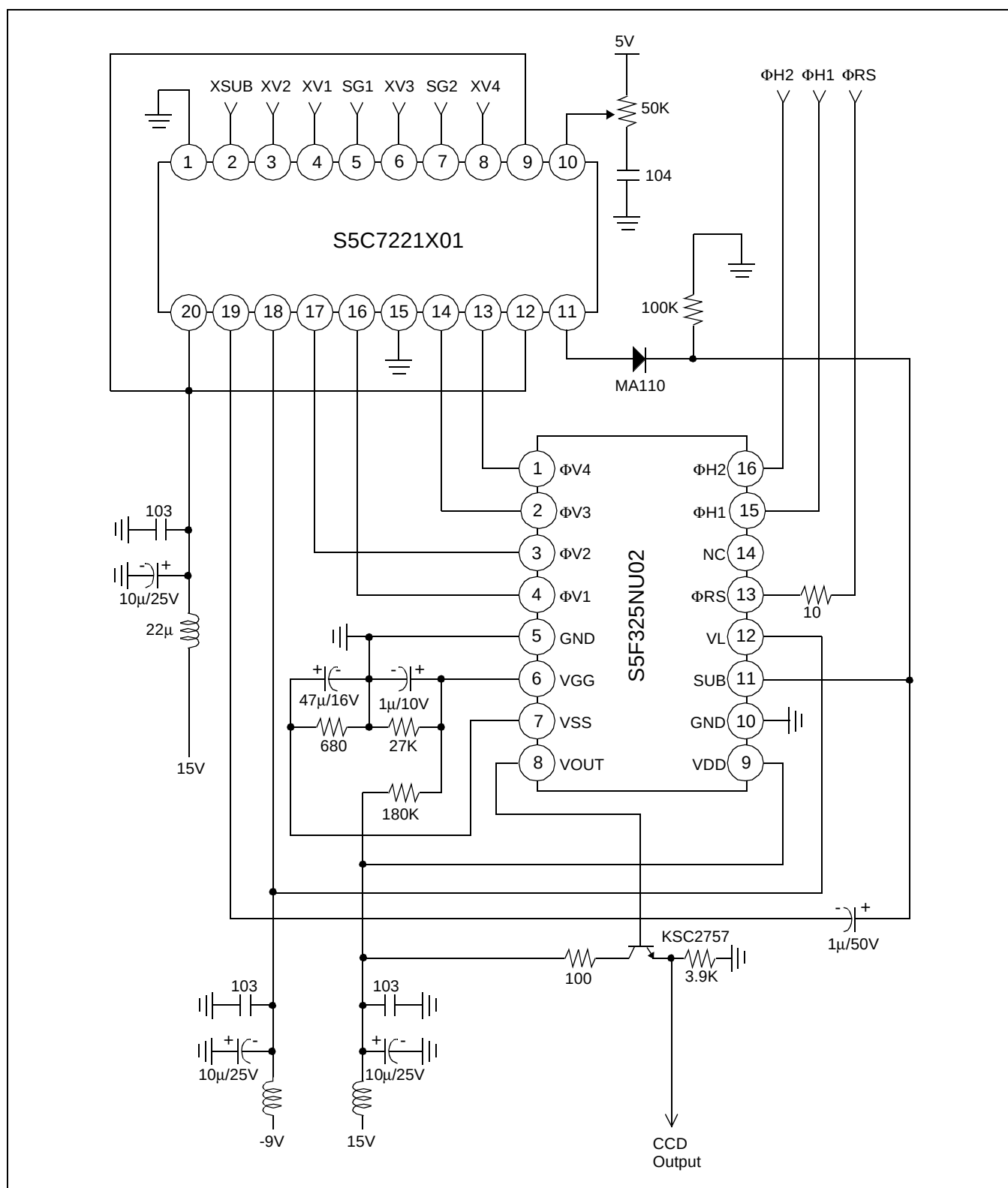
Figure 3. Application Circuits
