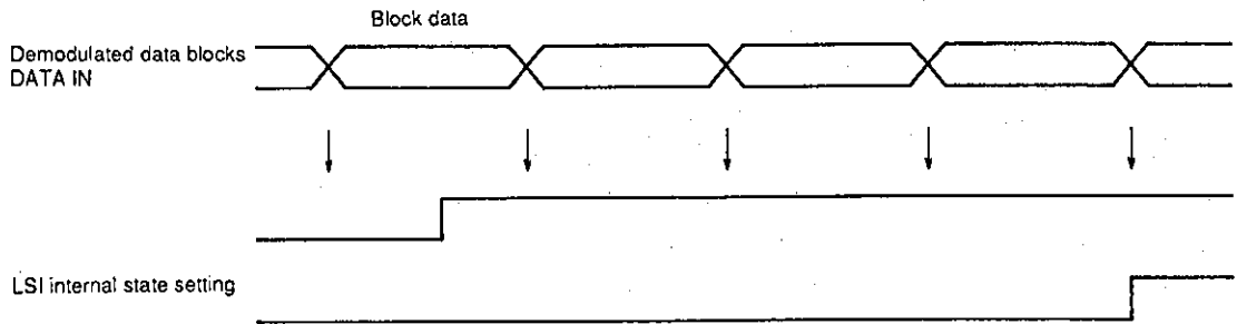
Pin Read-In Timing following Synchronization Detection
