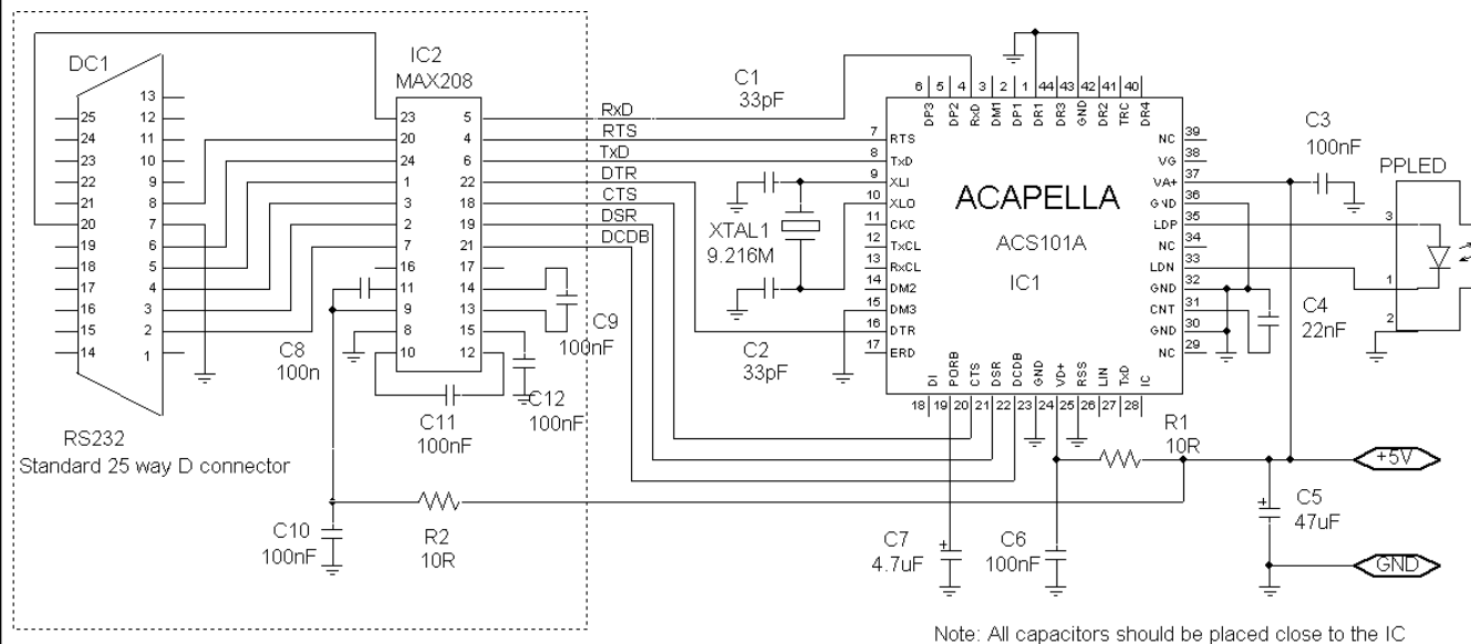
Figure 4. Typical application circuit for linking two PCs via a Single Fiber Optic Cable
