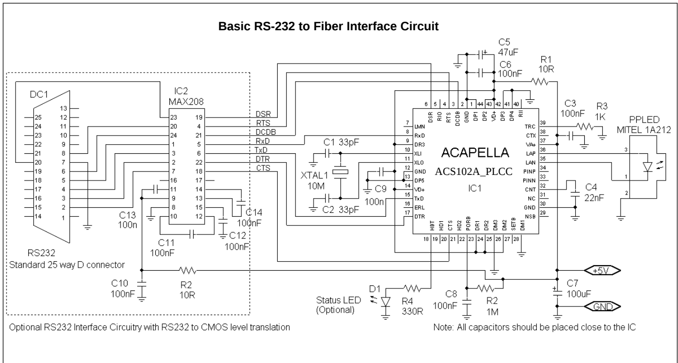
Figure 4. Typical application circuit for linking two PC Serial Ports via a Single Fiber Optic Cable using Ping-Pong LEDs. This diagram shows a PLCC44 package being used. The TQFP44 package option can be used with the same component layout.
