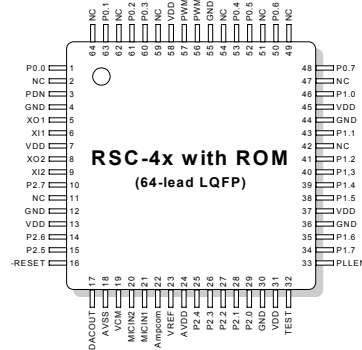
64-lead LQFP
