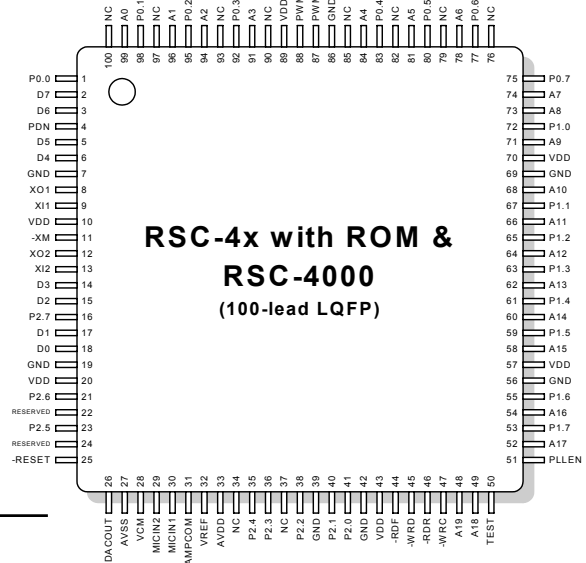
100-lead LQFP
