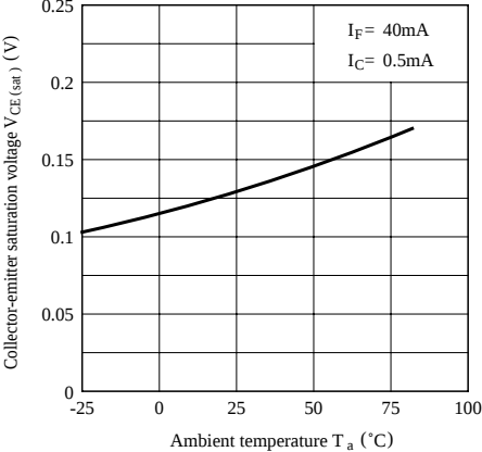
Fig. 8 Collector-emitter Saturation Voltage Ambient Temperature
