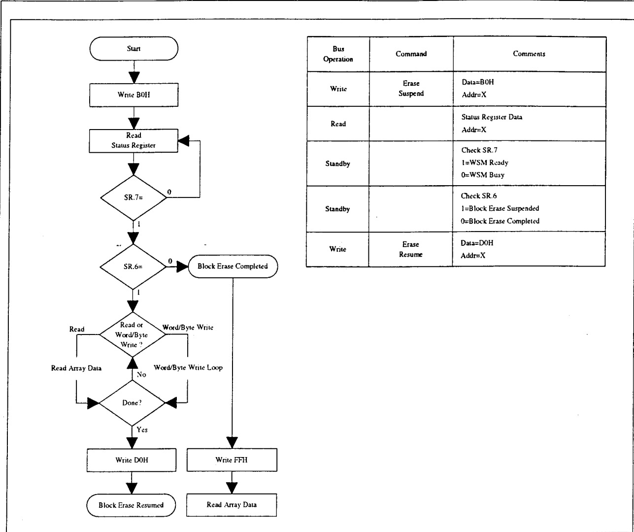
Figure 8. Block Erase Suspend/Resume Flowchart
