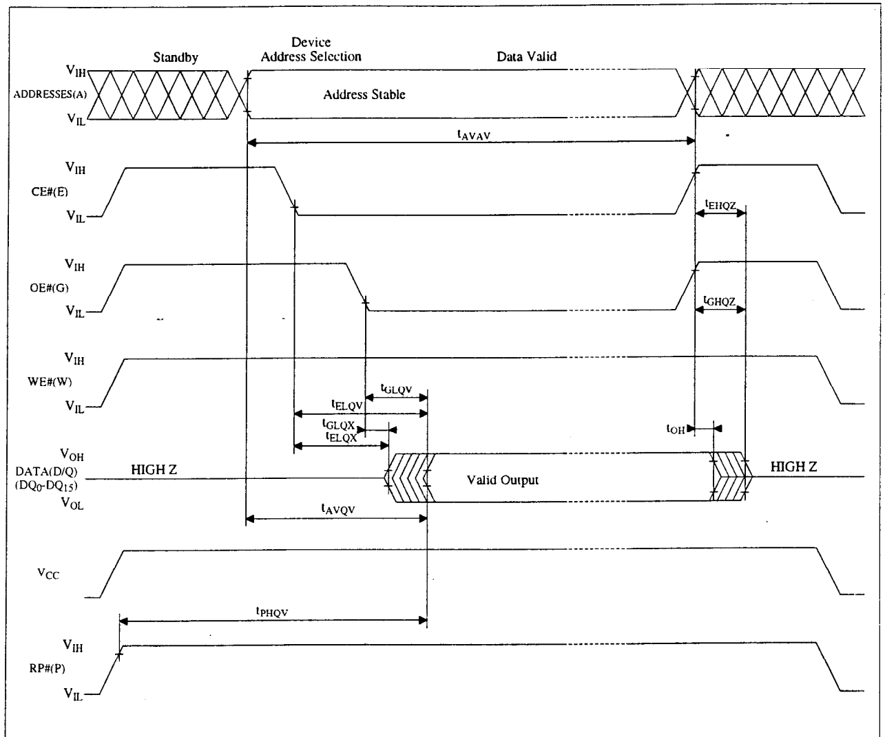
Figure 14. AC Waveform for Read Operations
