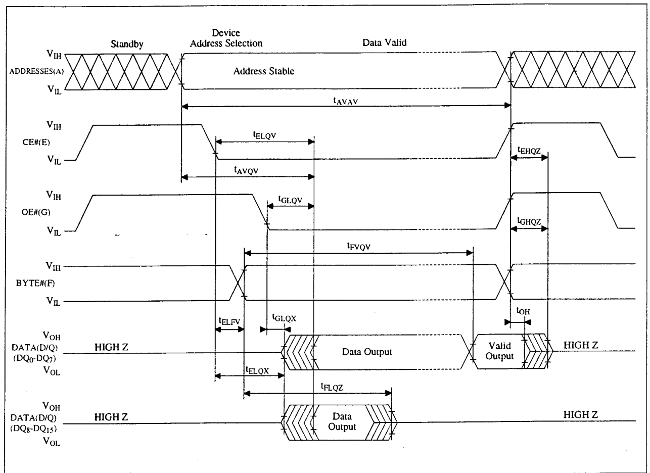
Figure 15. BYTE# timing Waveform
