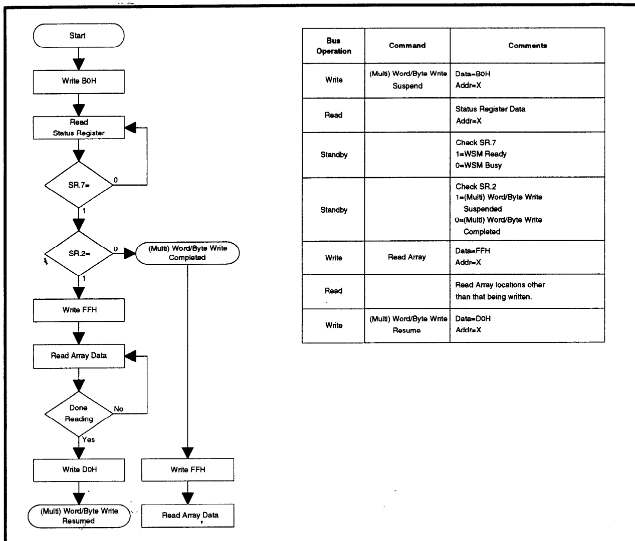
Figure 11. (Multi) Word/Byte Write Suspend/Resume Flowchart
