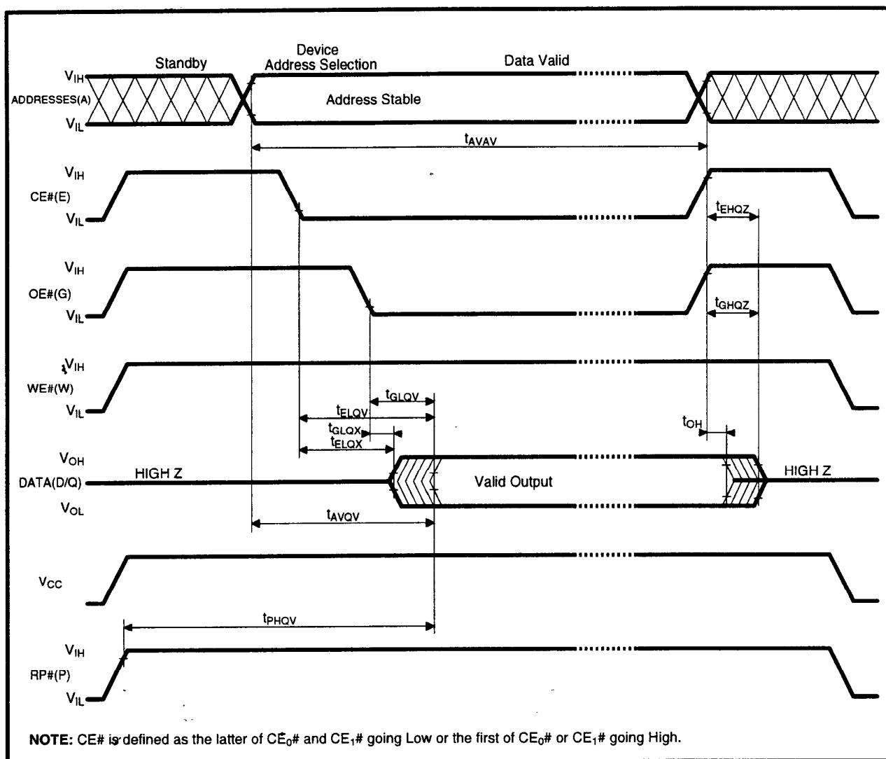
Figure 17. AC Waveform for Read Operations
