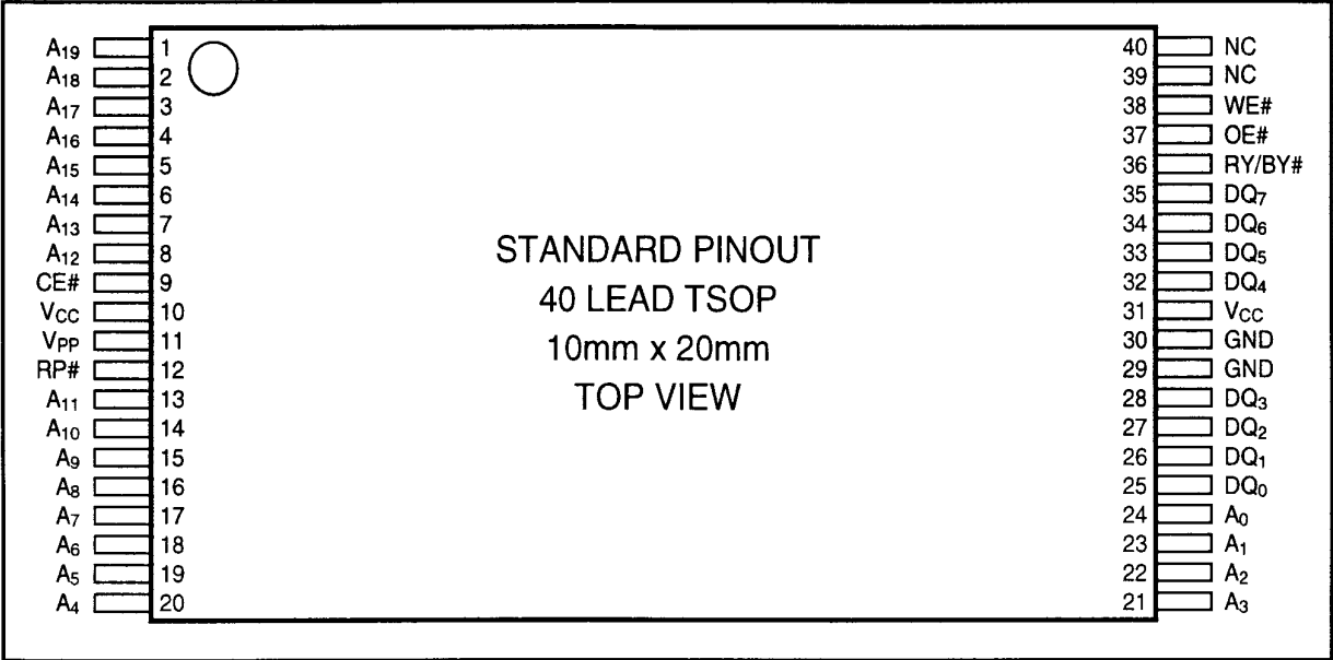
Figure 2. TSOP Lead Configuration
