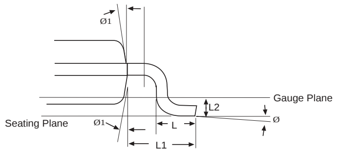
VIEW C
