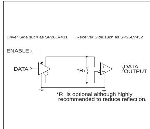
Figure 21. Two-Wire Balanced Systems, RS-422
